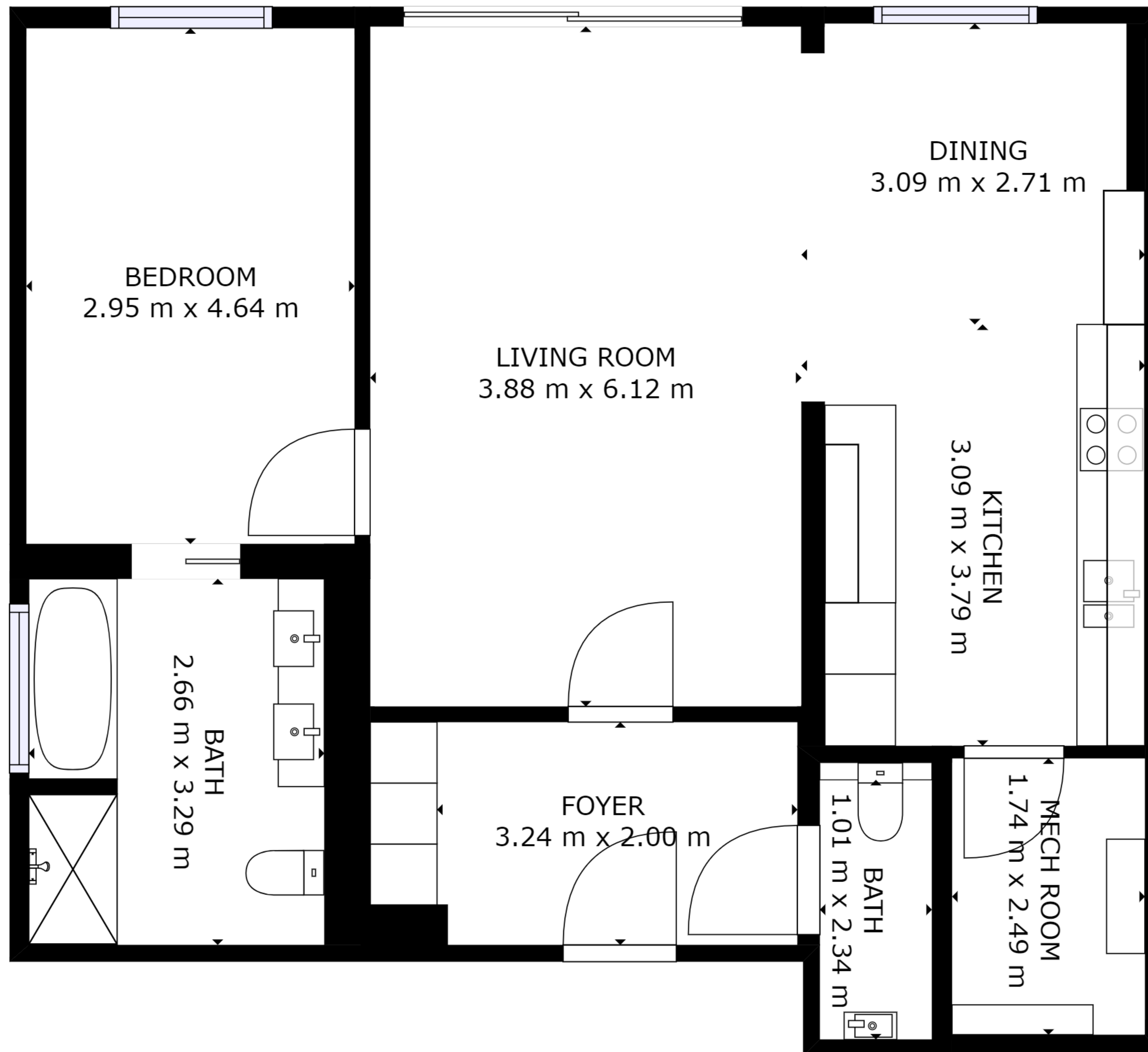
FLOOR 1
