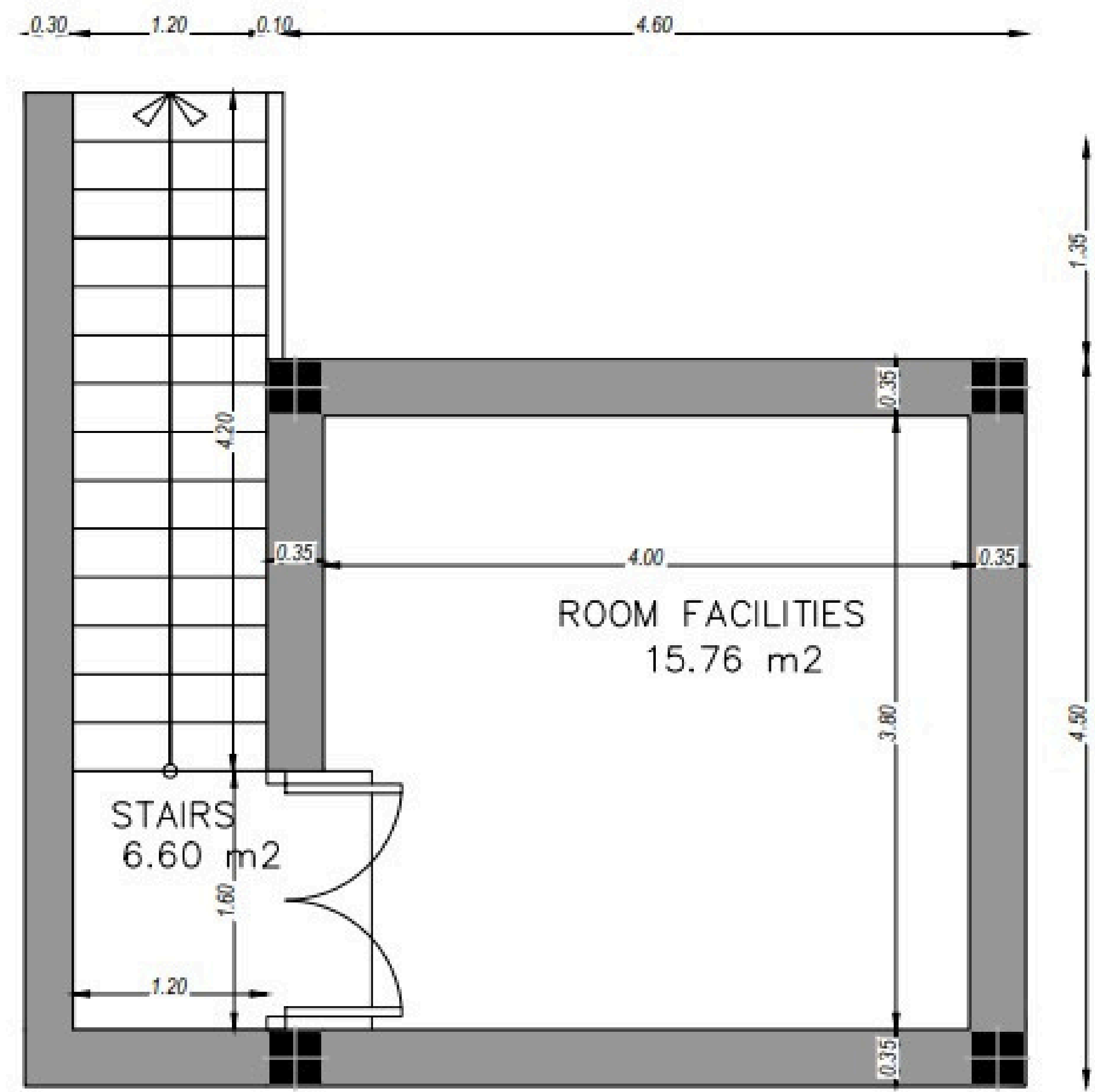
BASEMENT 23.98 M2
