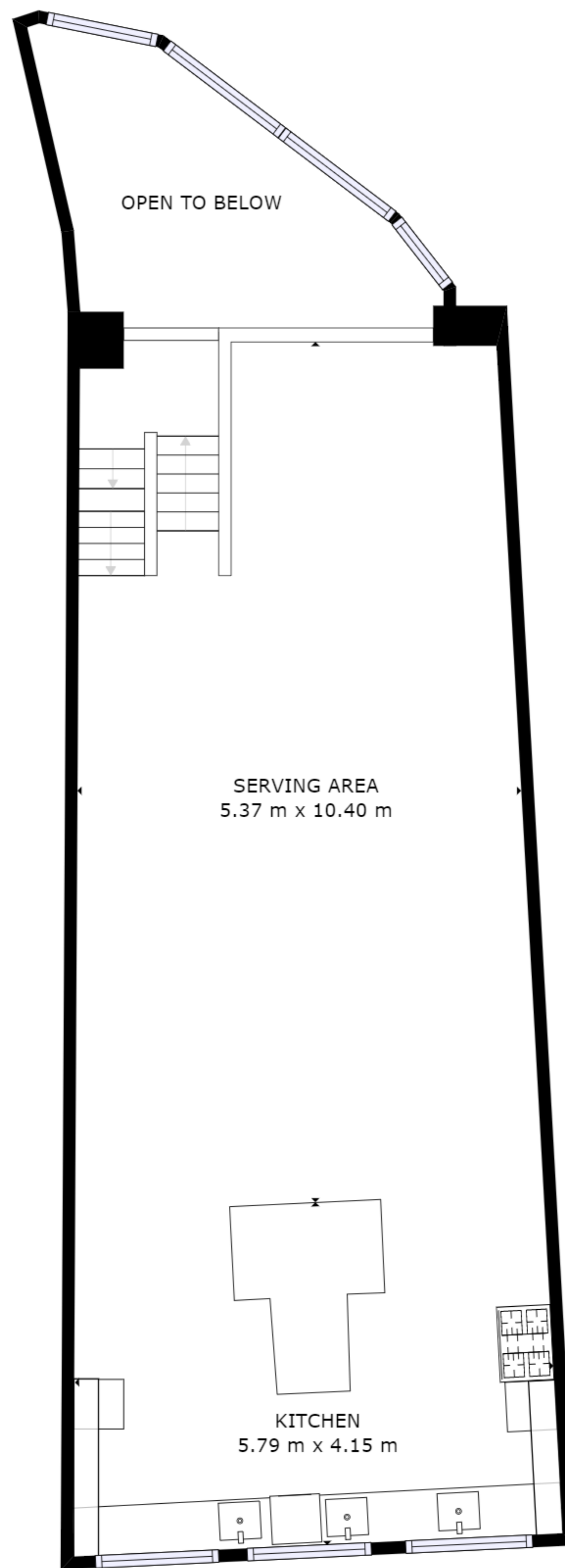
FLOOR 2
