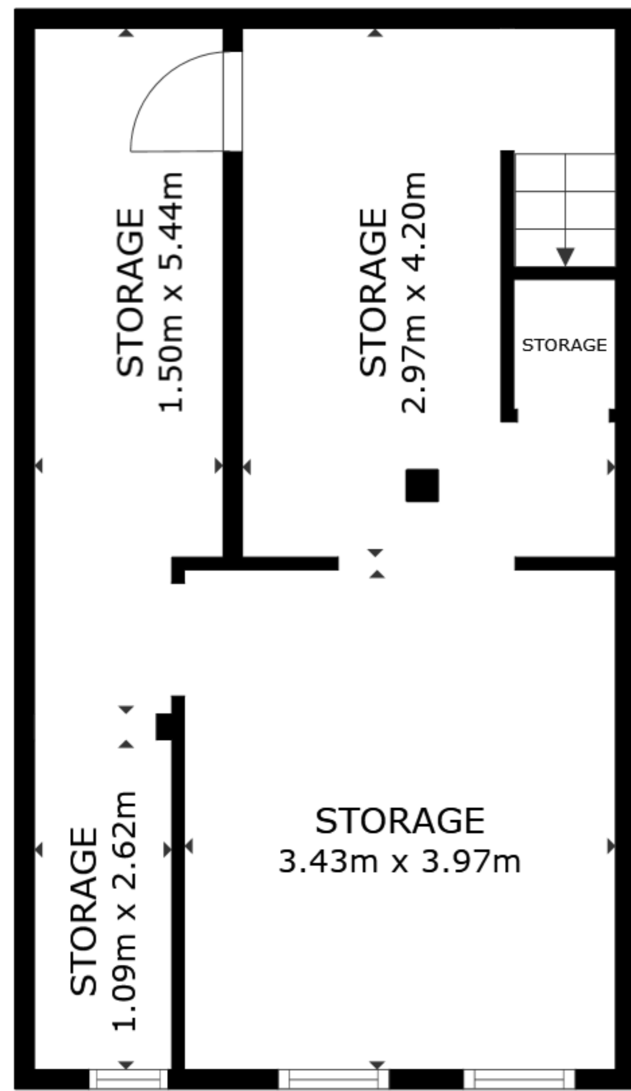
FLOOR 1
