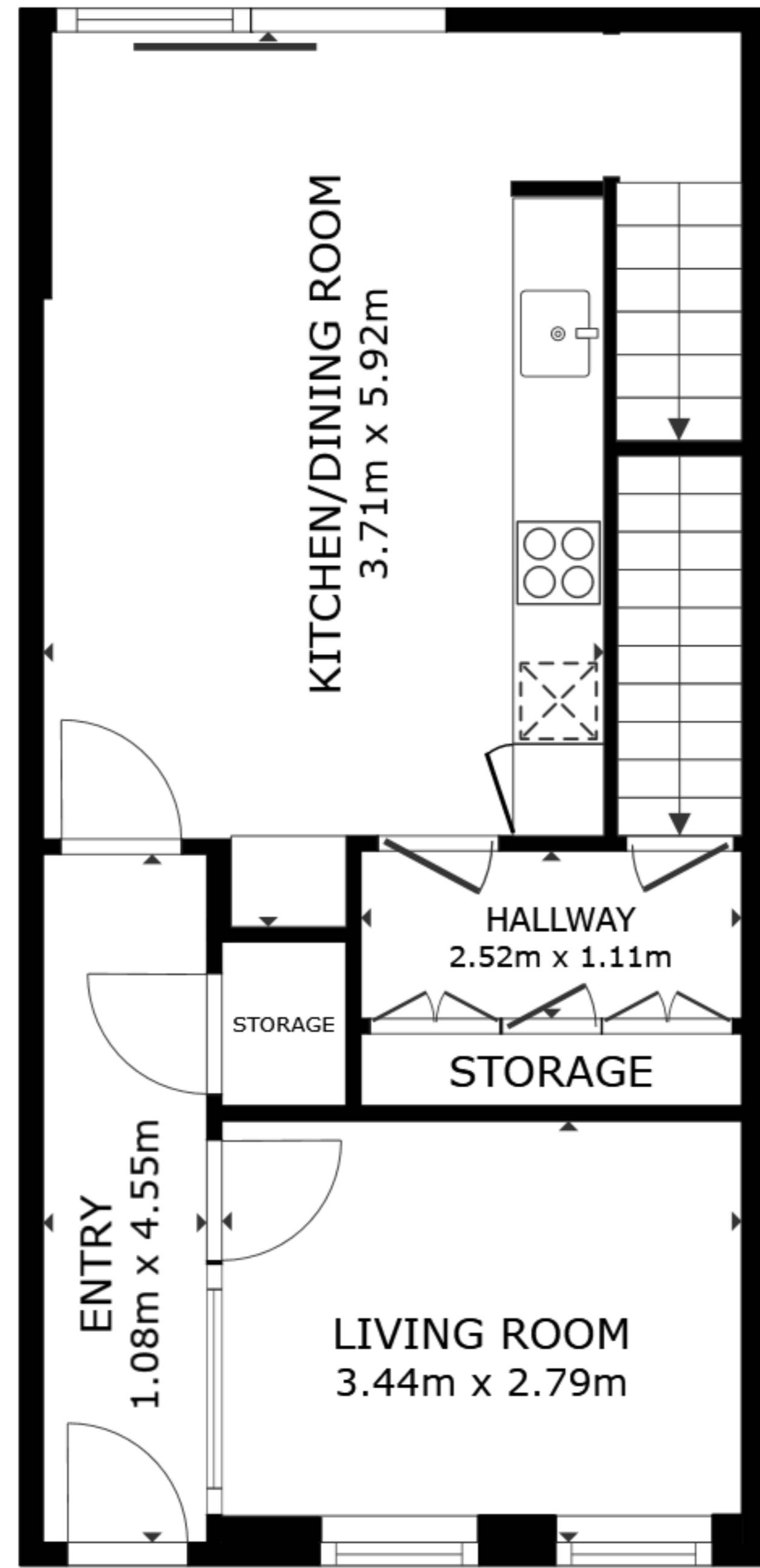
FLOOR 2
