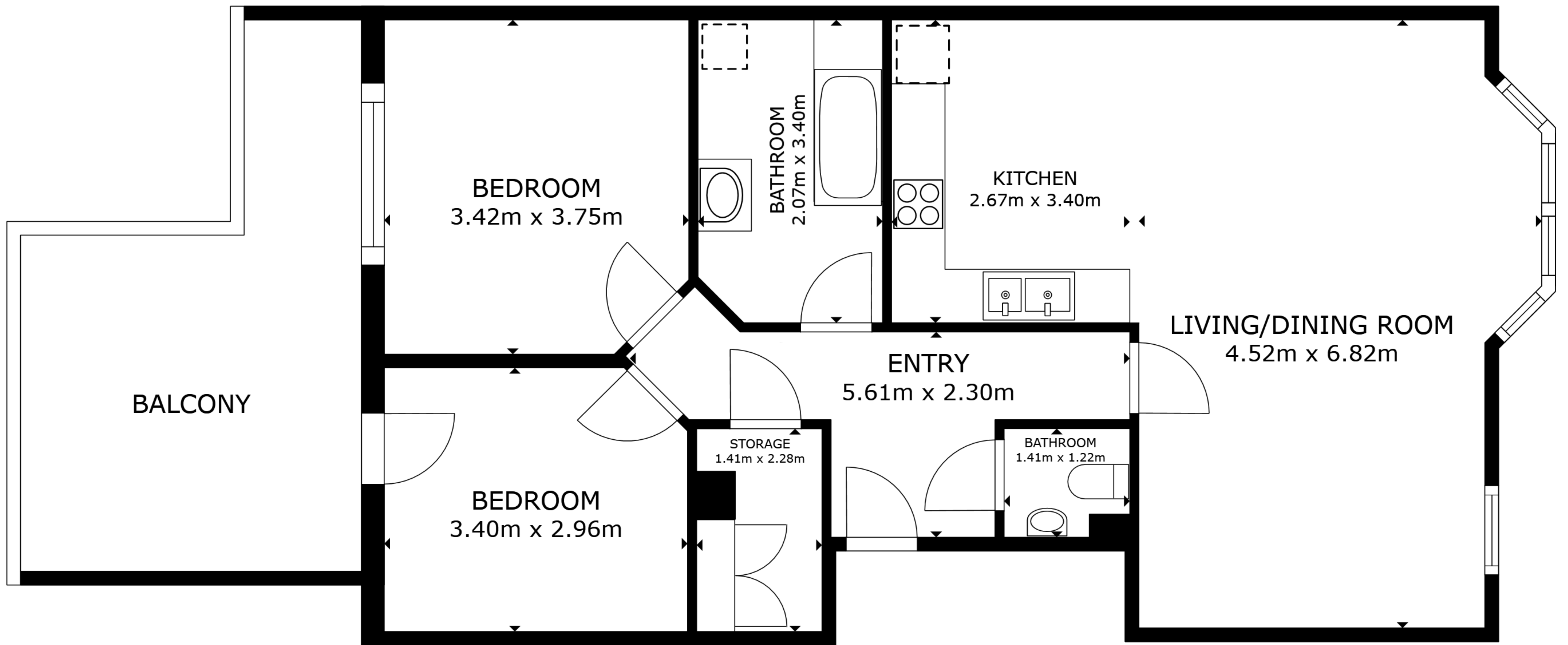
FLOOR PLAN
