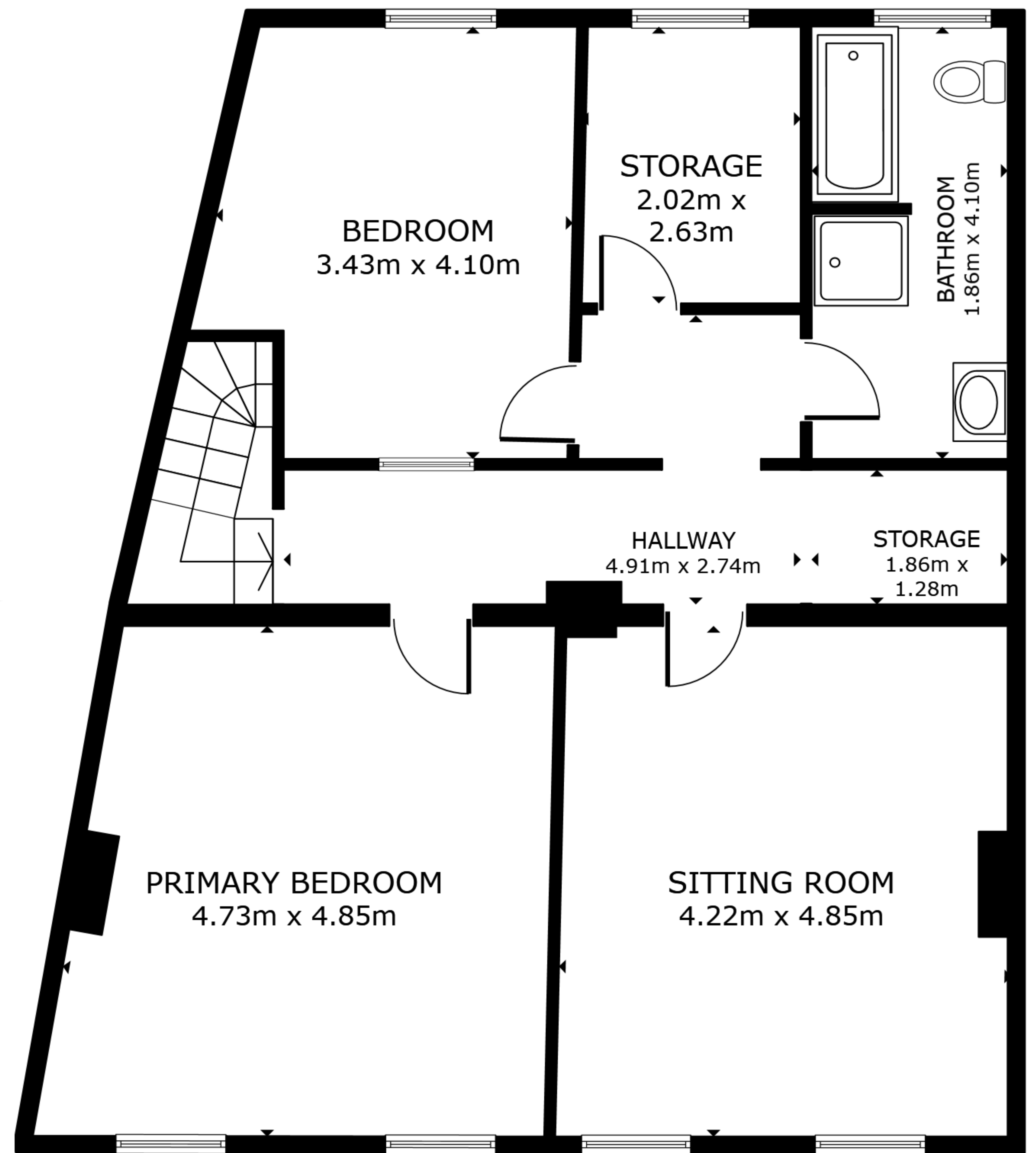
FLOOR 1
