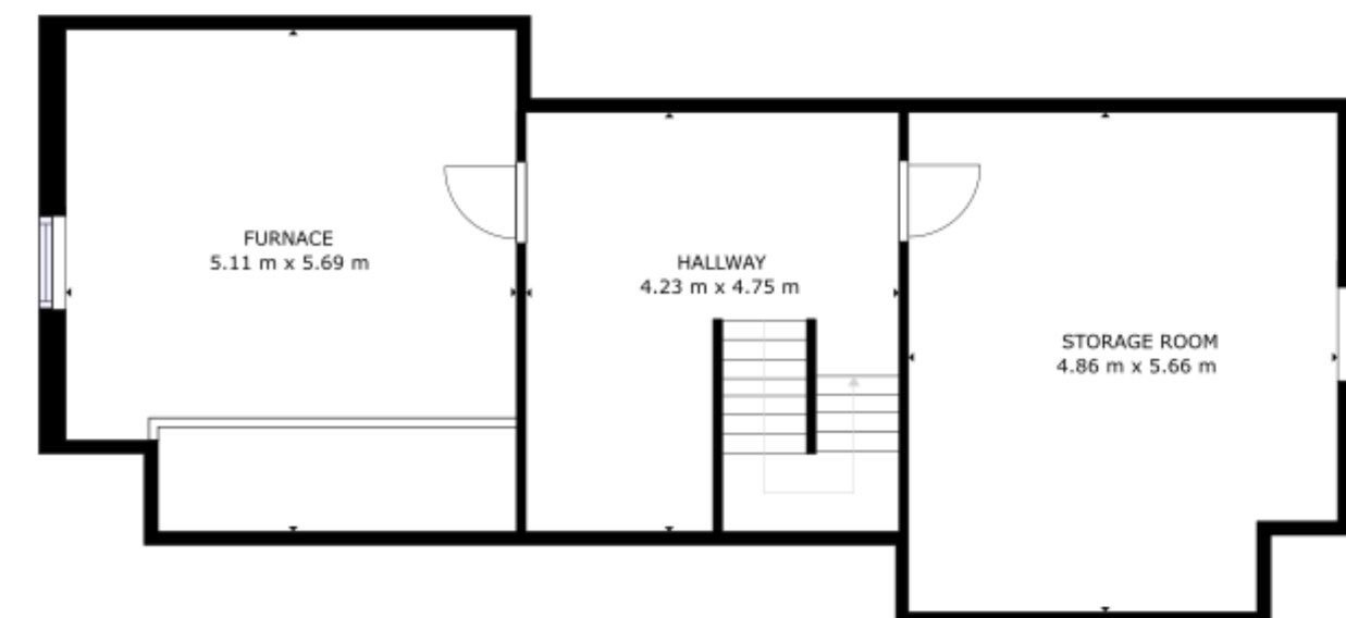
FLOOR 1
