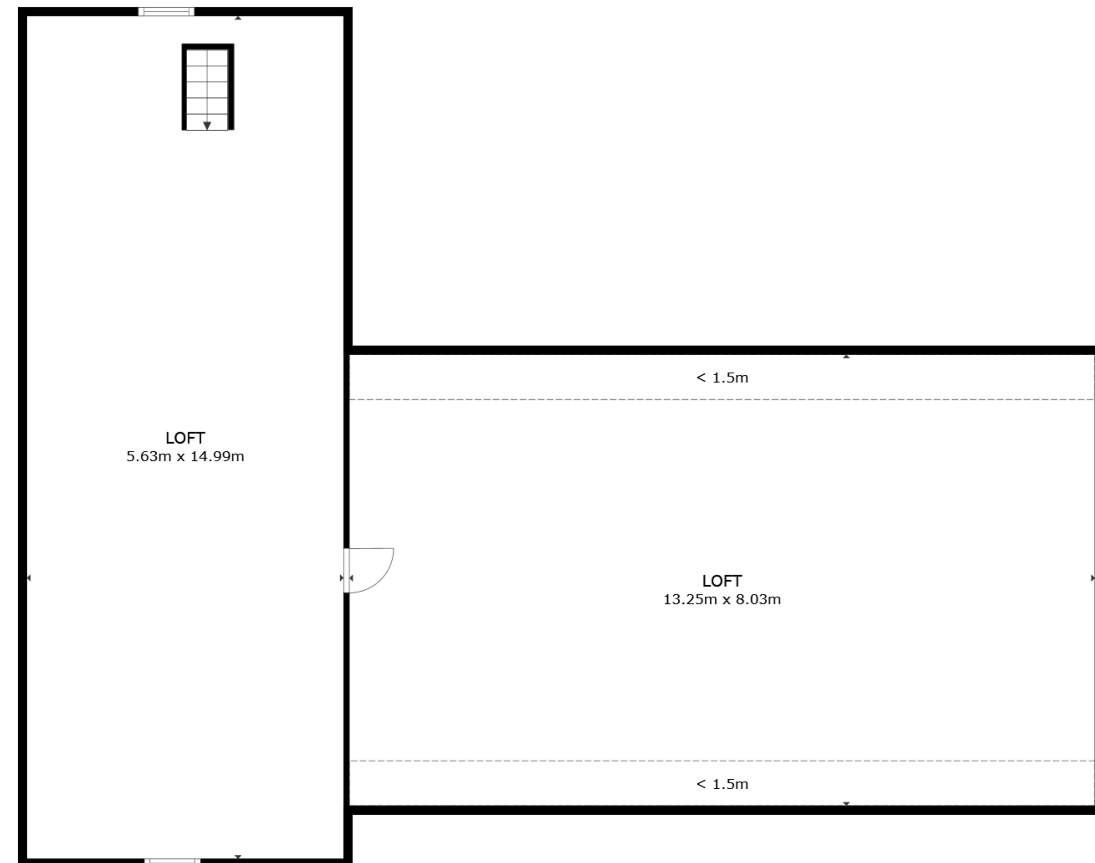
FLOOR 2
