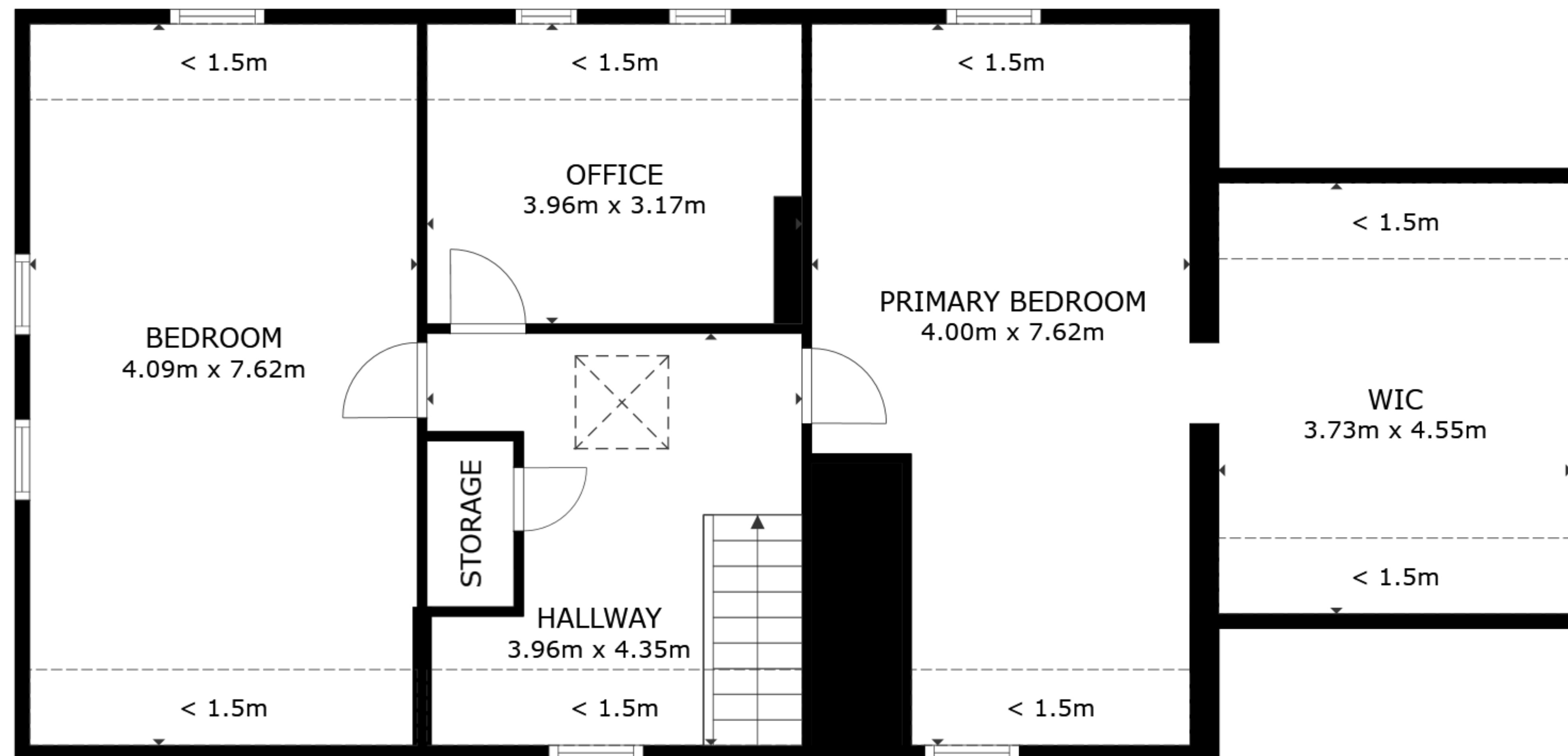
FLOOR 2
