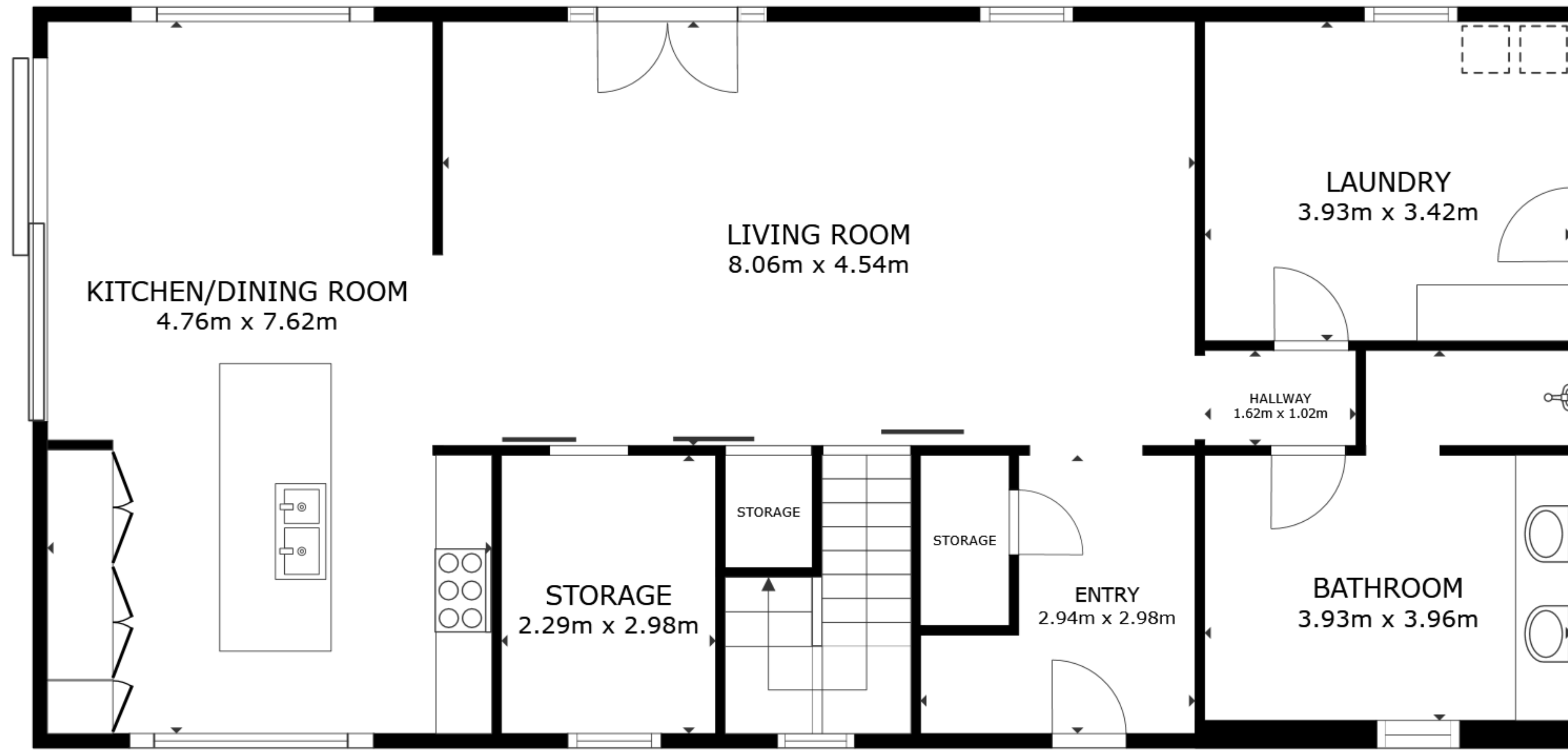
FLOOR 1
