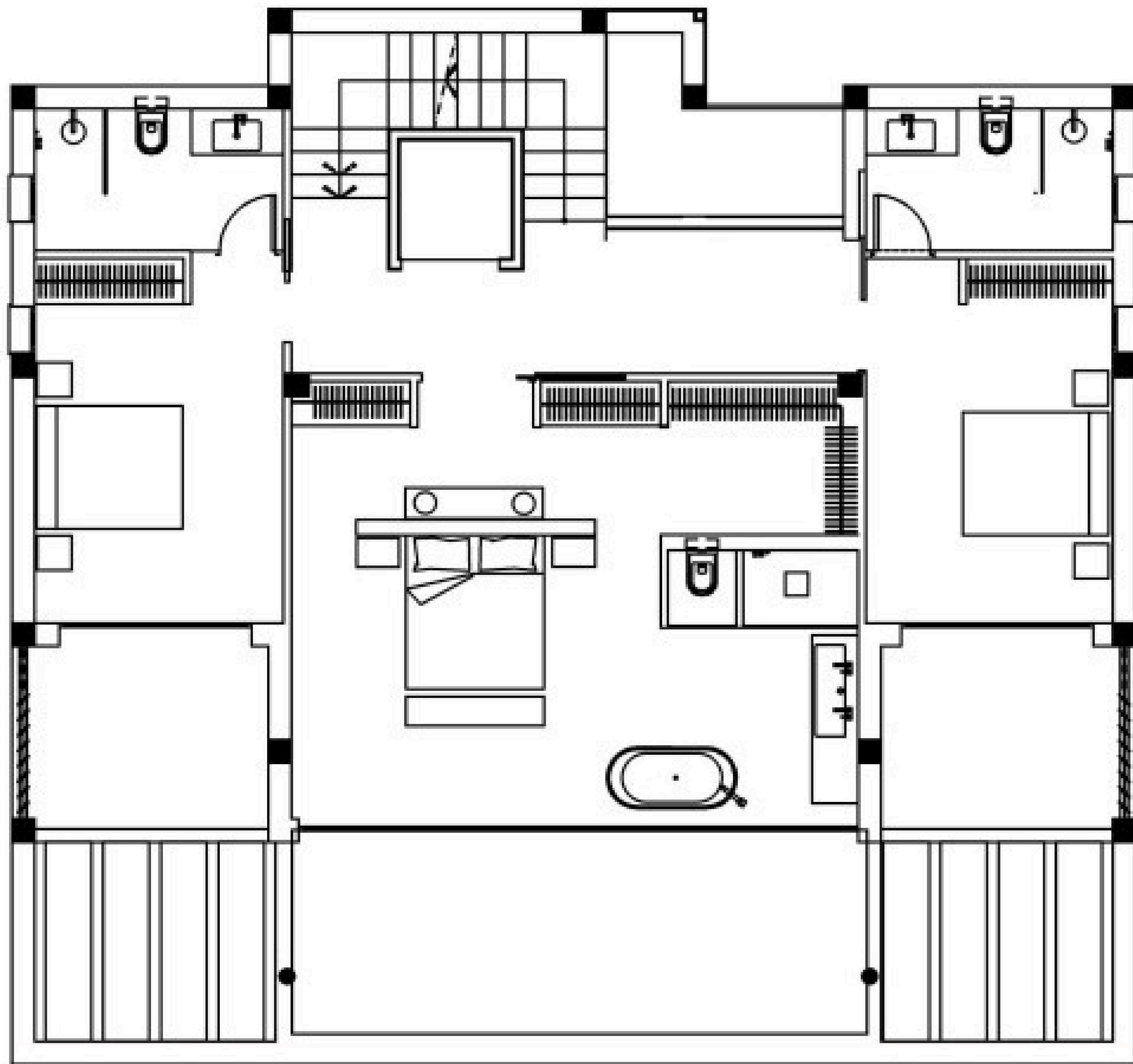
TOP FLOOR
