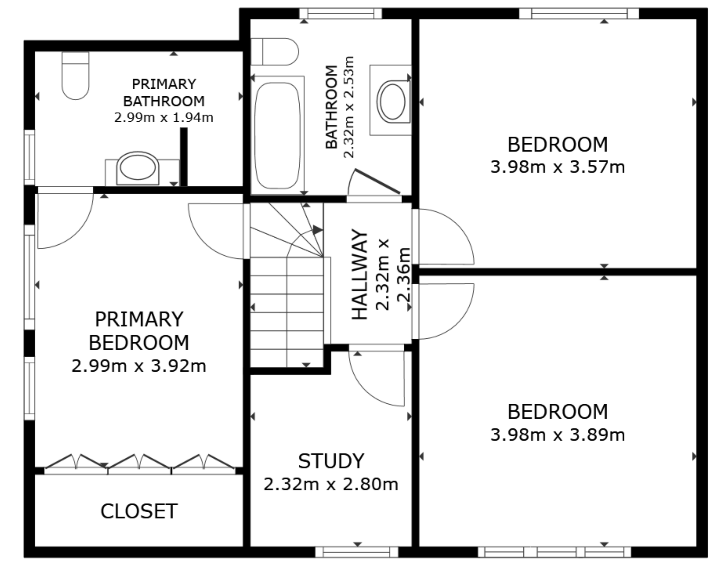
FLOOR 2
