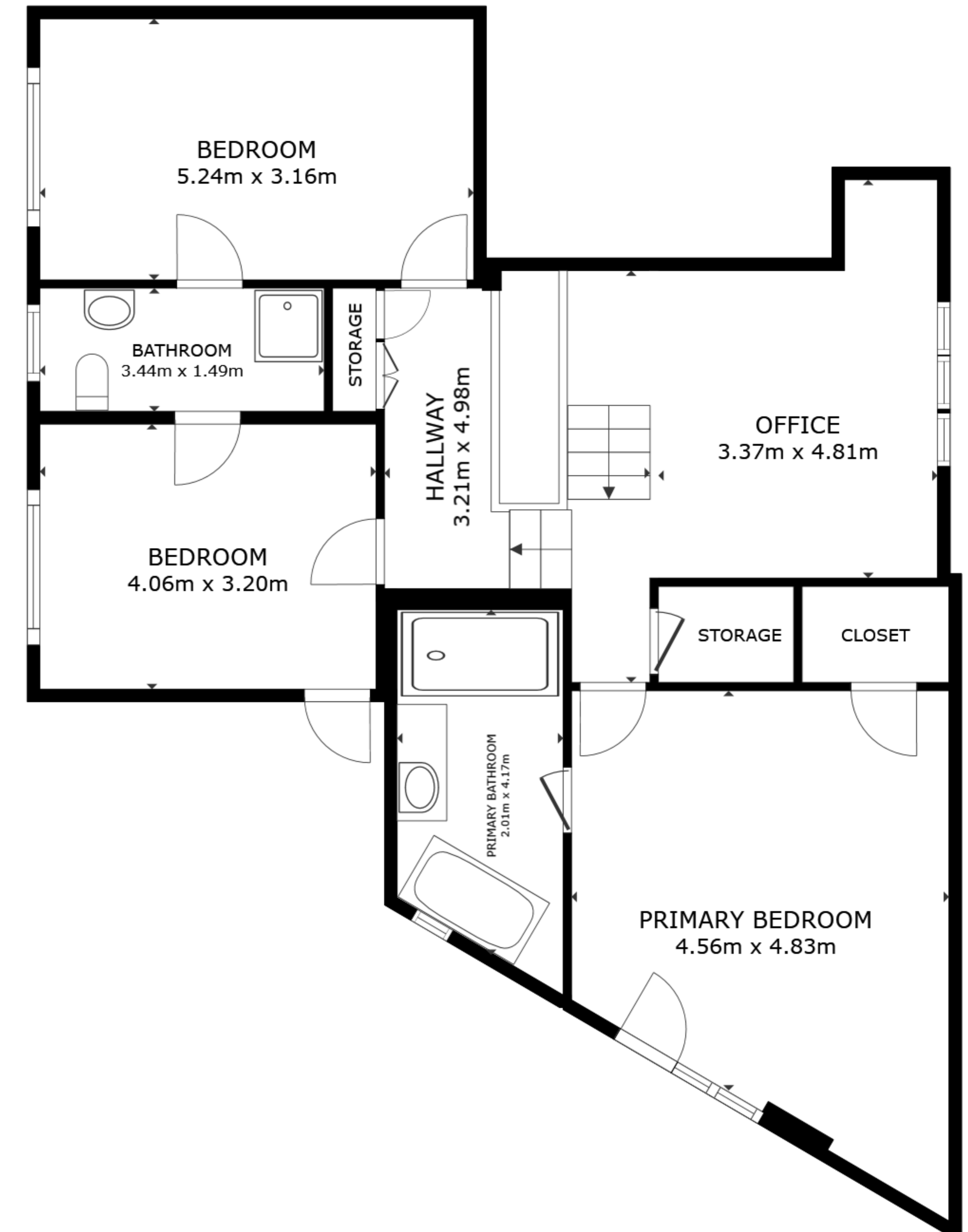
FLOOR 2
