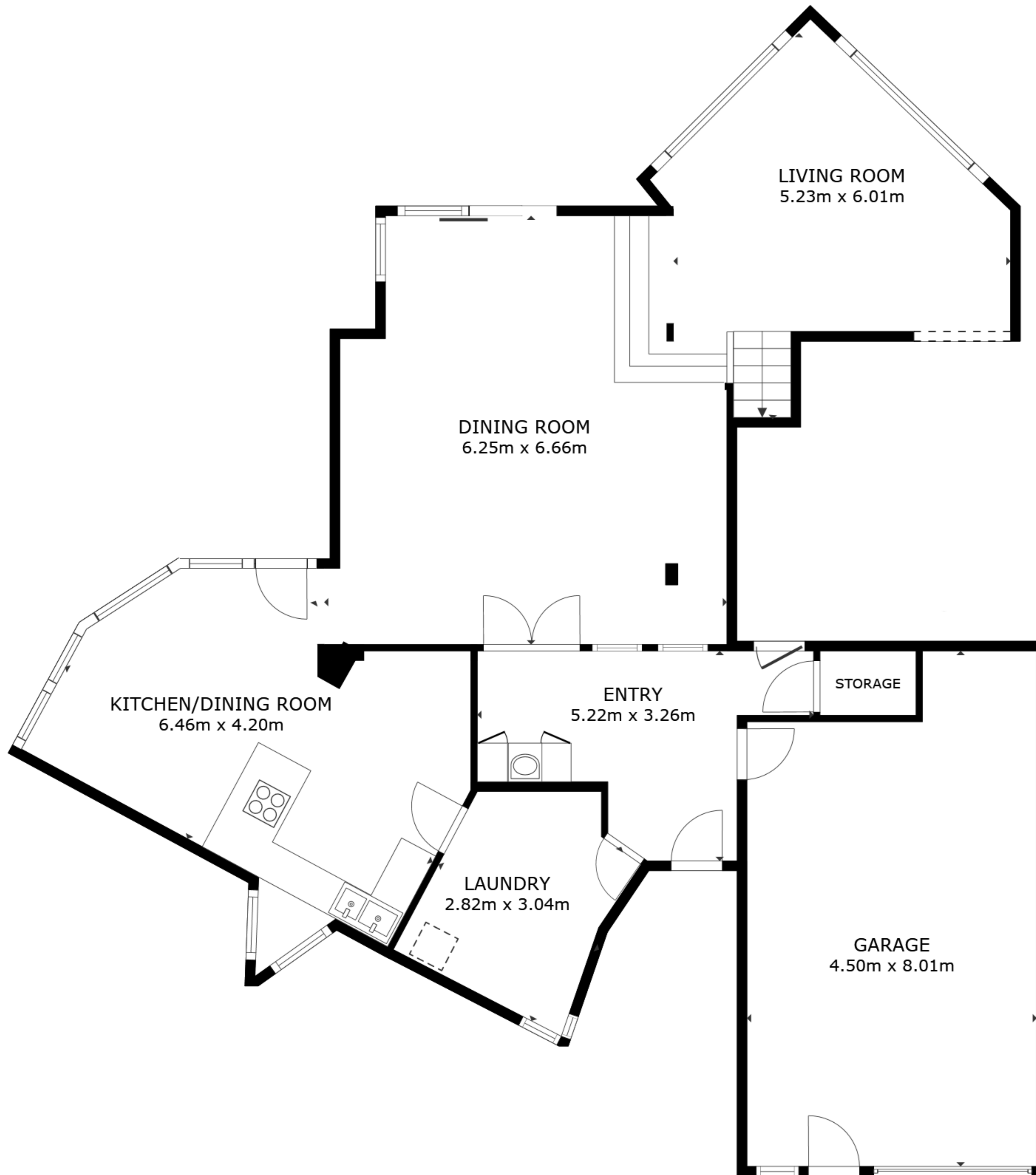
FLOOR 1
