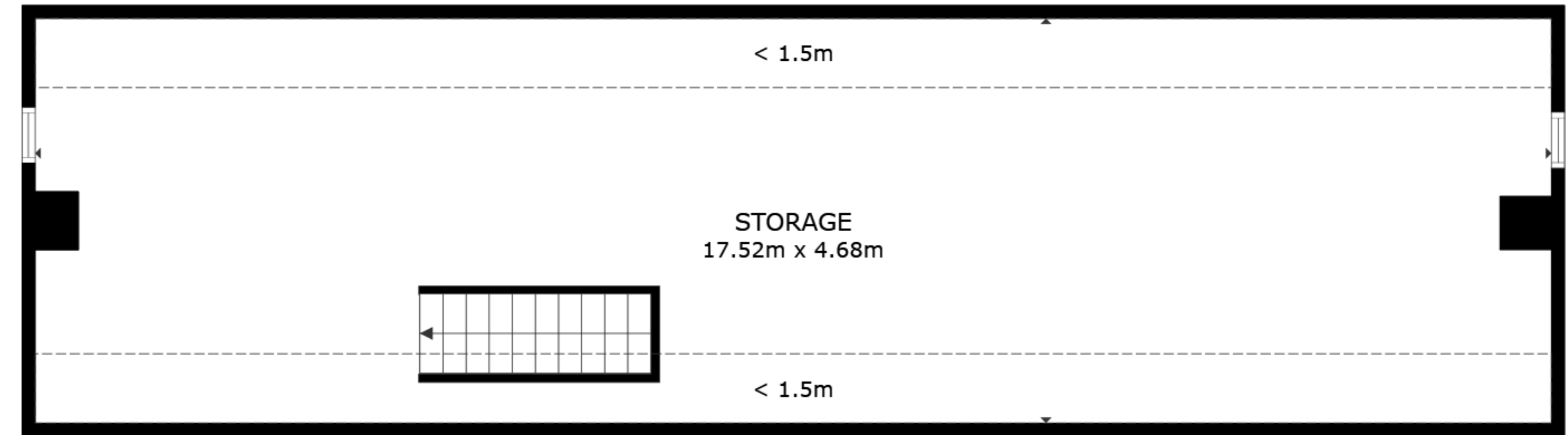
FLOOR 3
