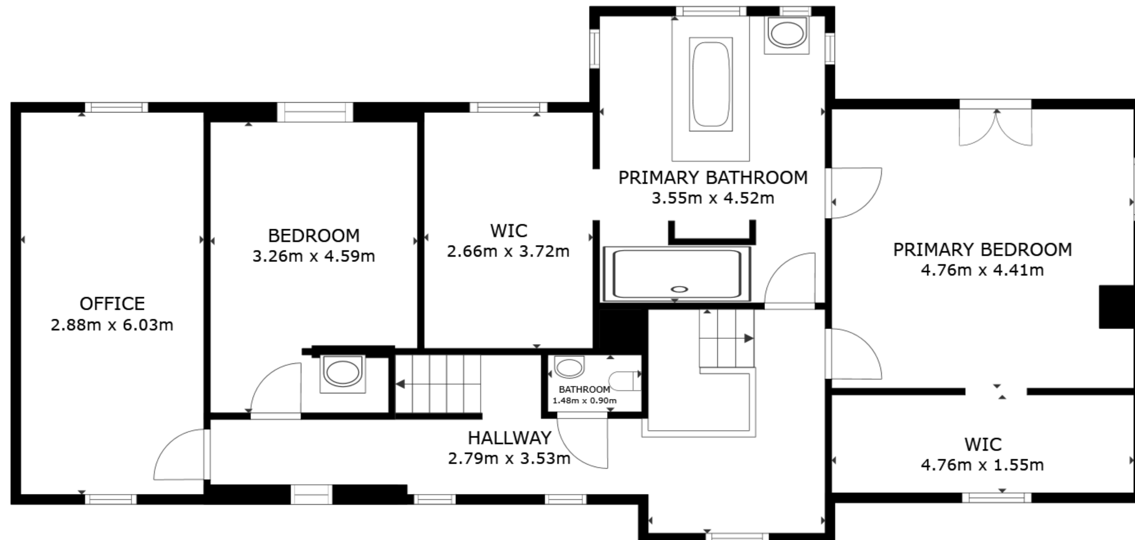
FLOOR 2
