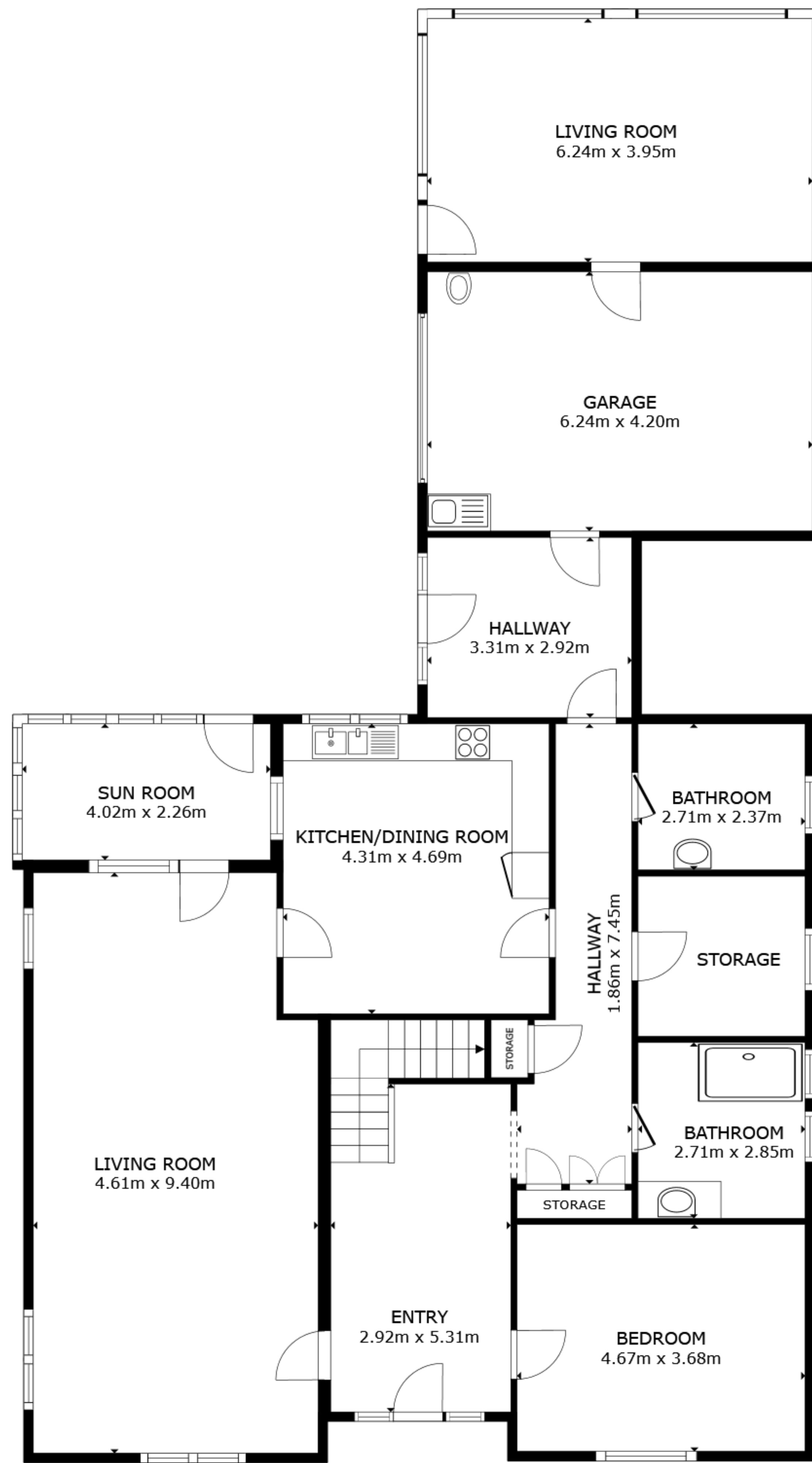
FLOOR 1
