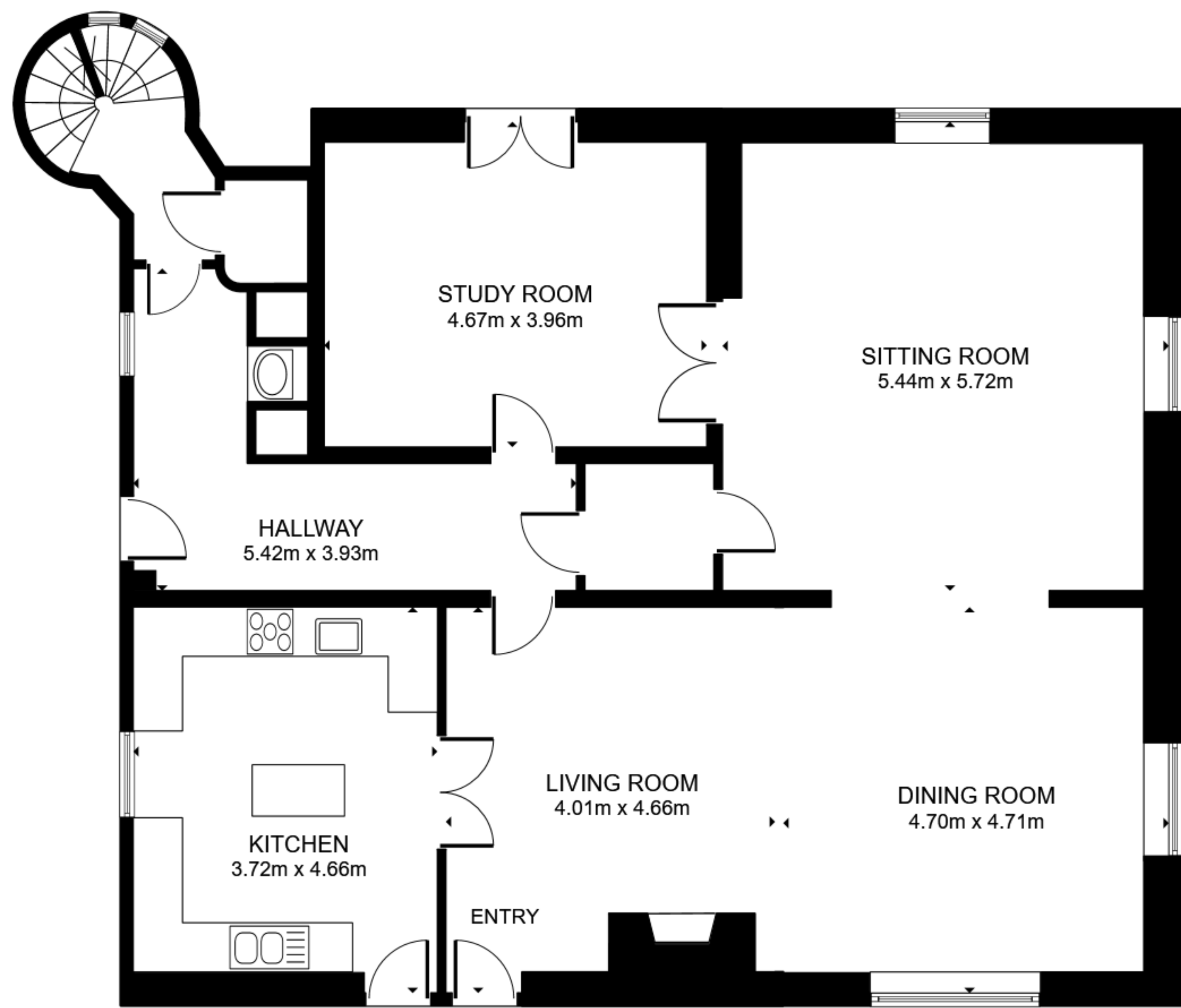
GROUND FLOOR
