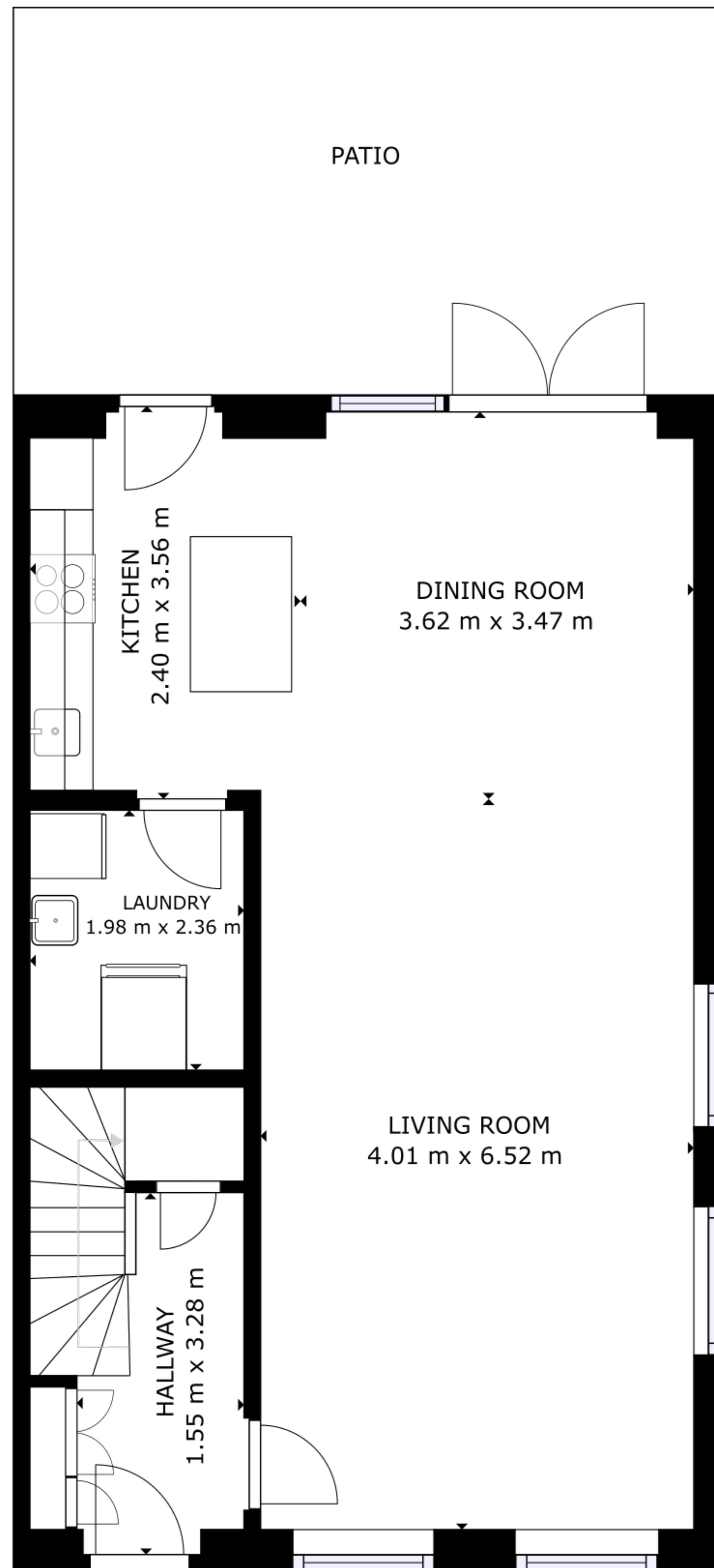
FLOOR 1
