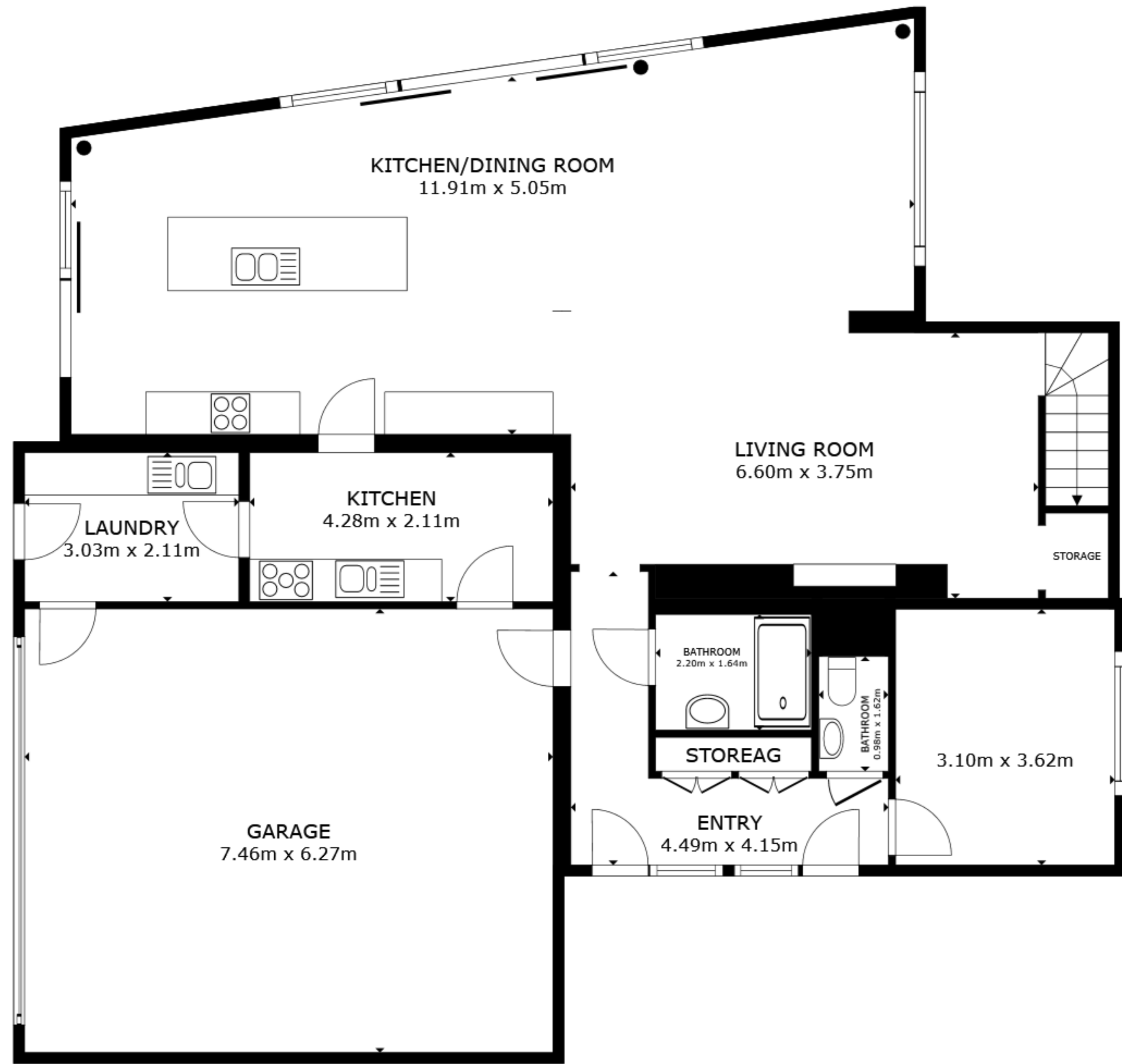
GROUND FLOOR
