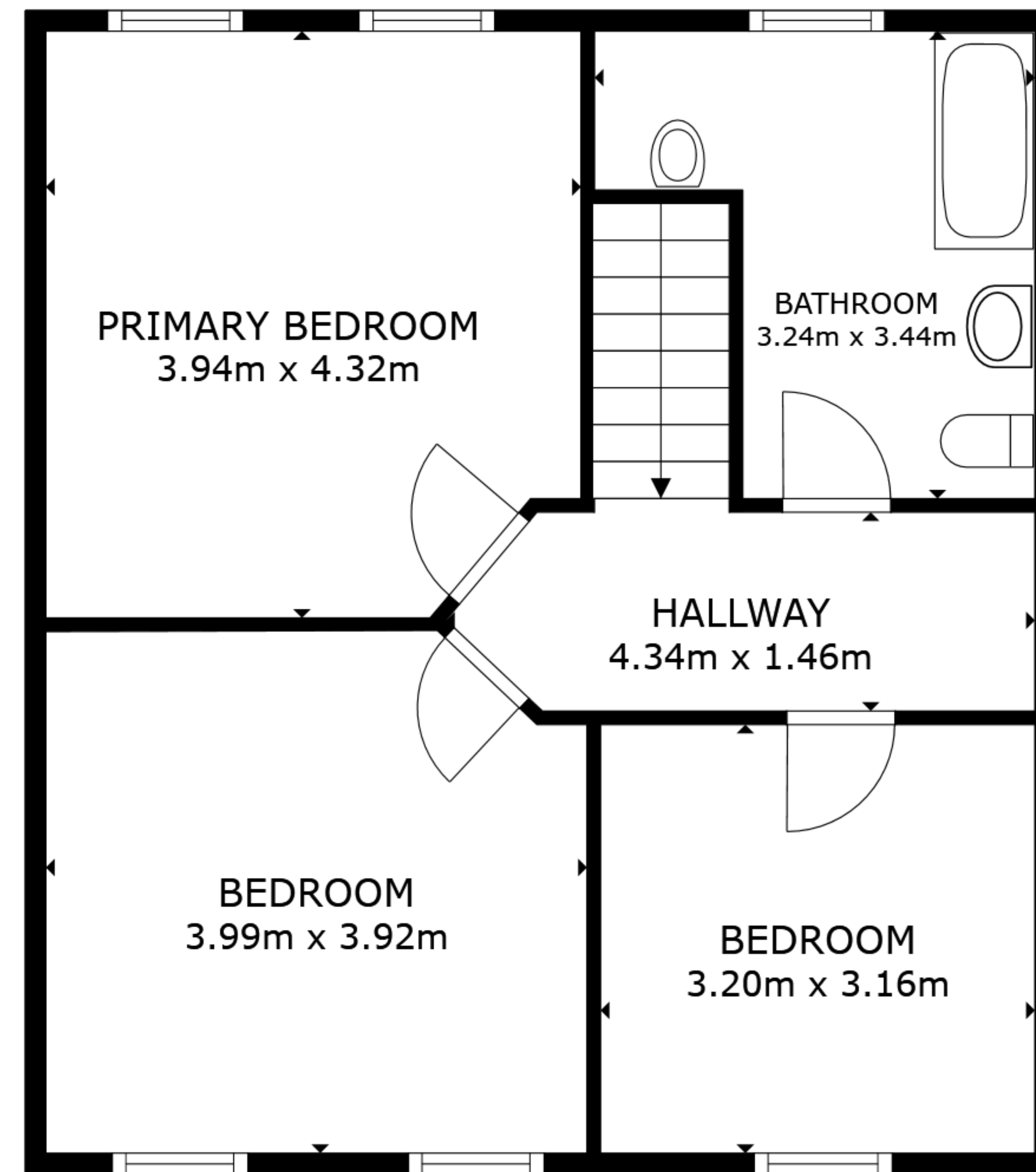
FLOOR 2
