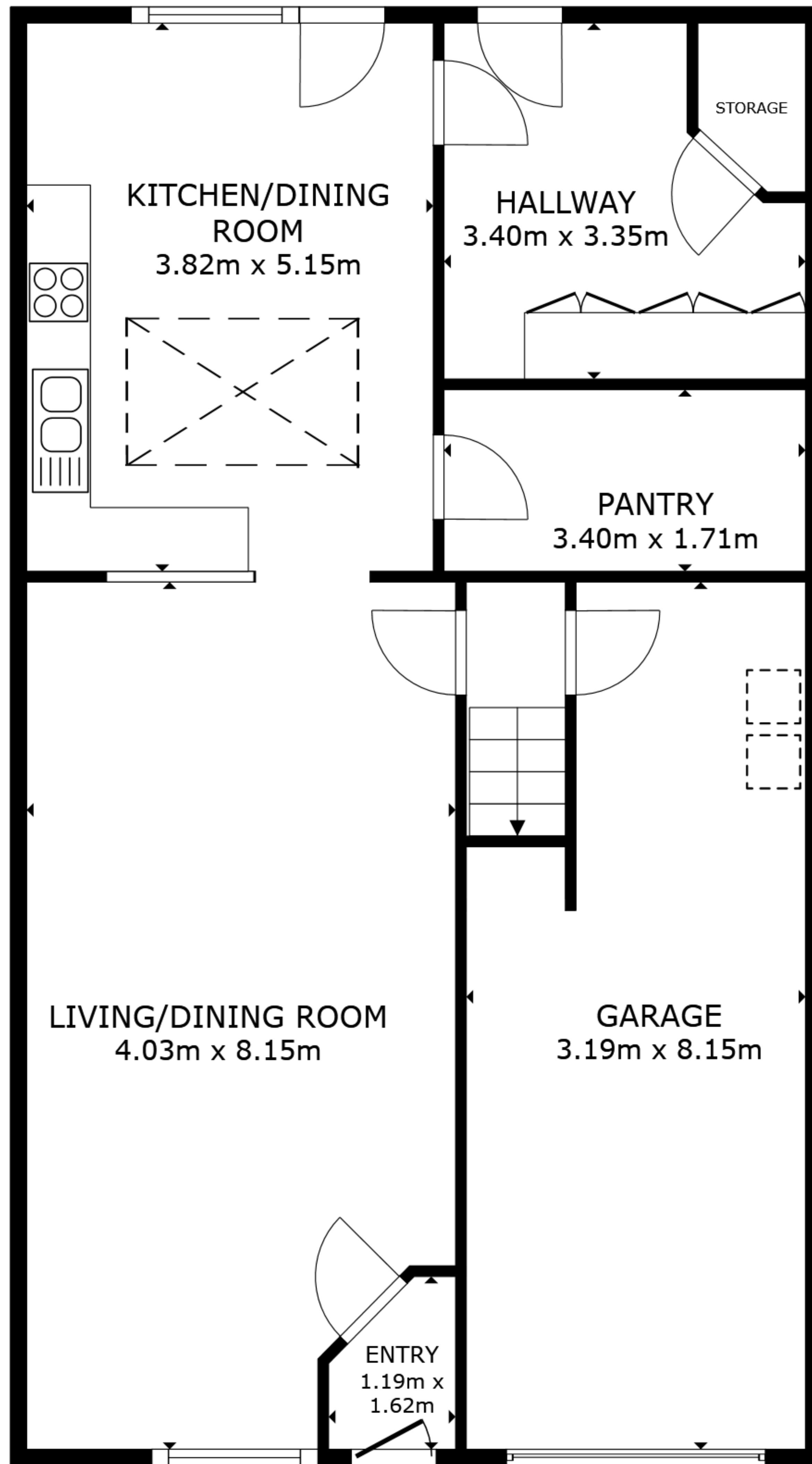
FLOOR 1
