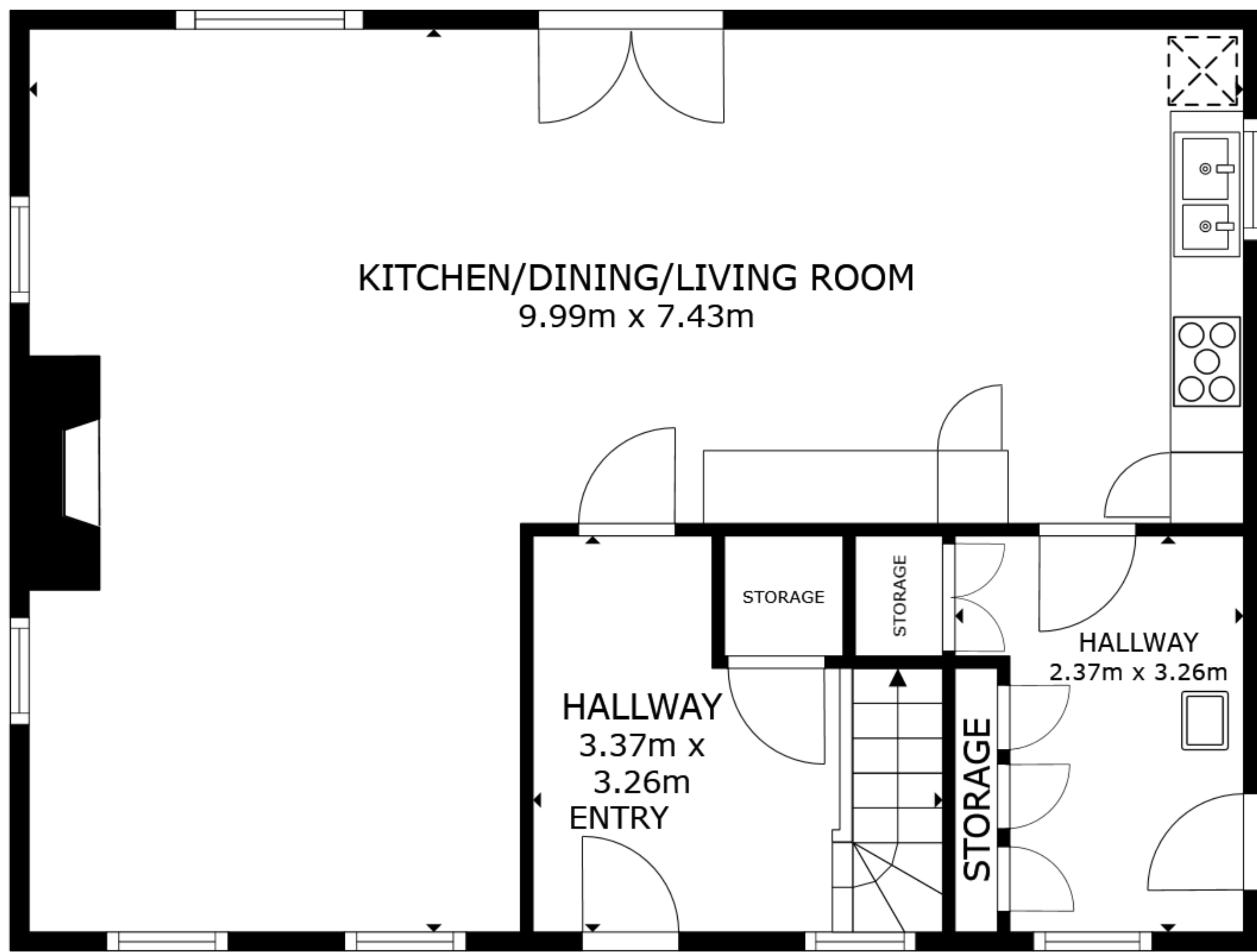
FLOOR 1
