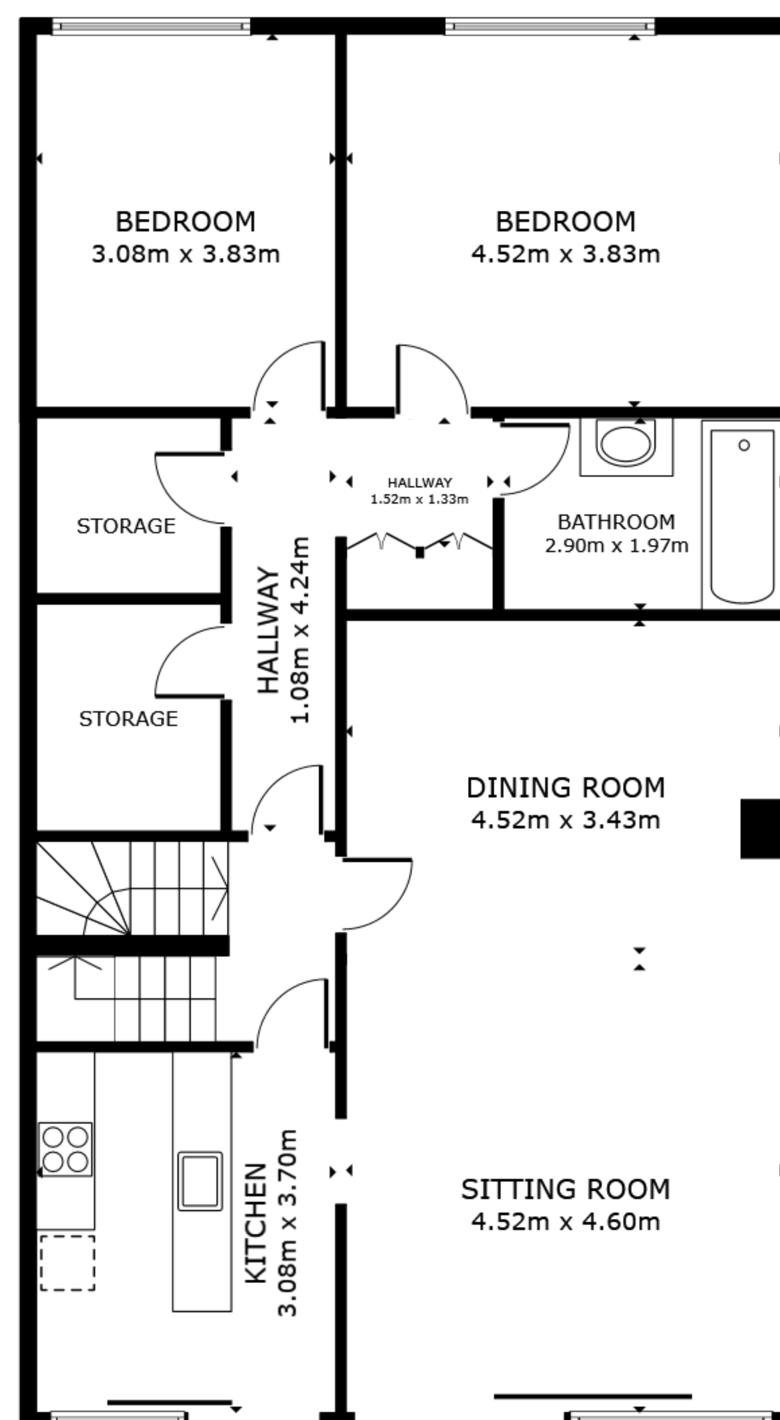
FLOOR 2
