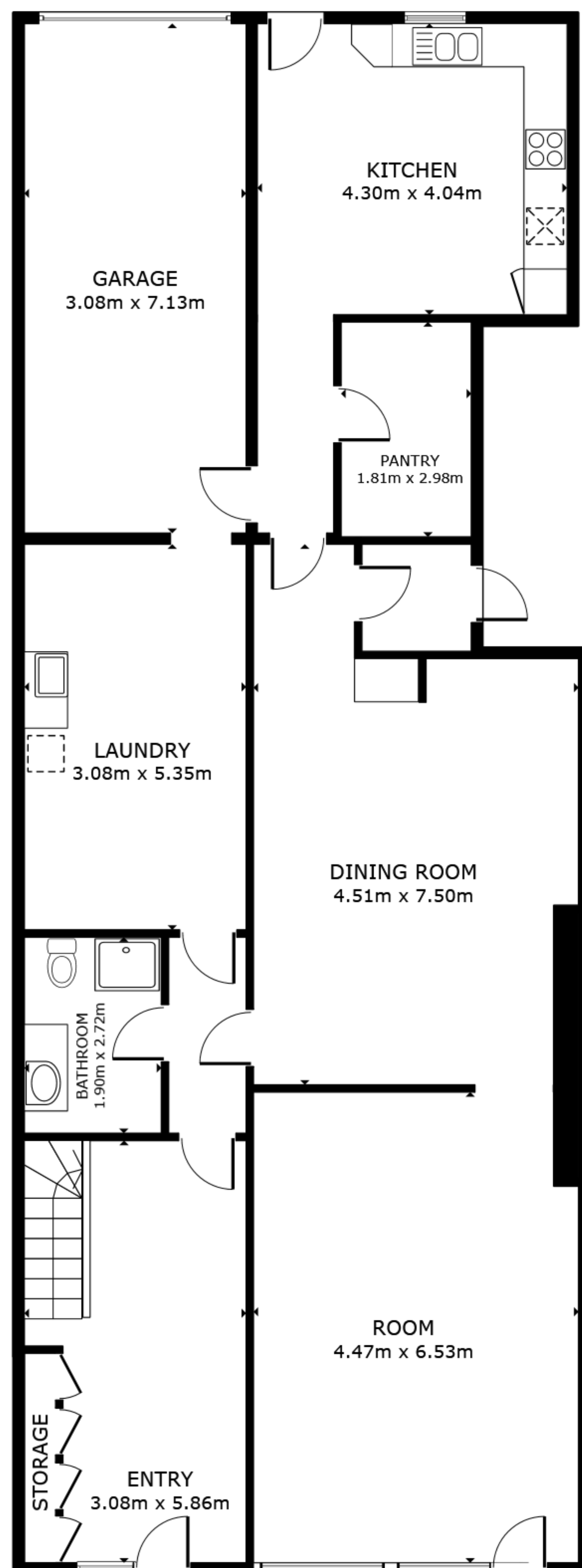
FLOOR 1
