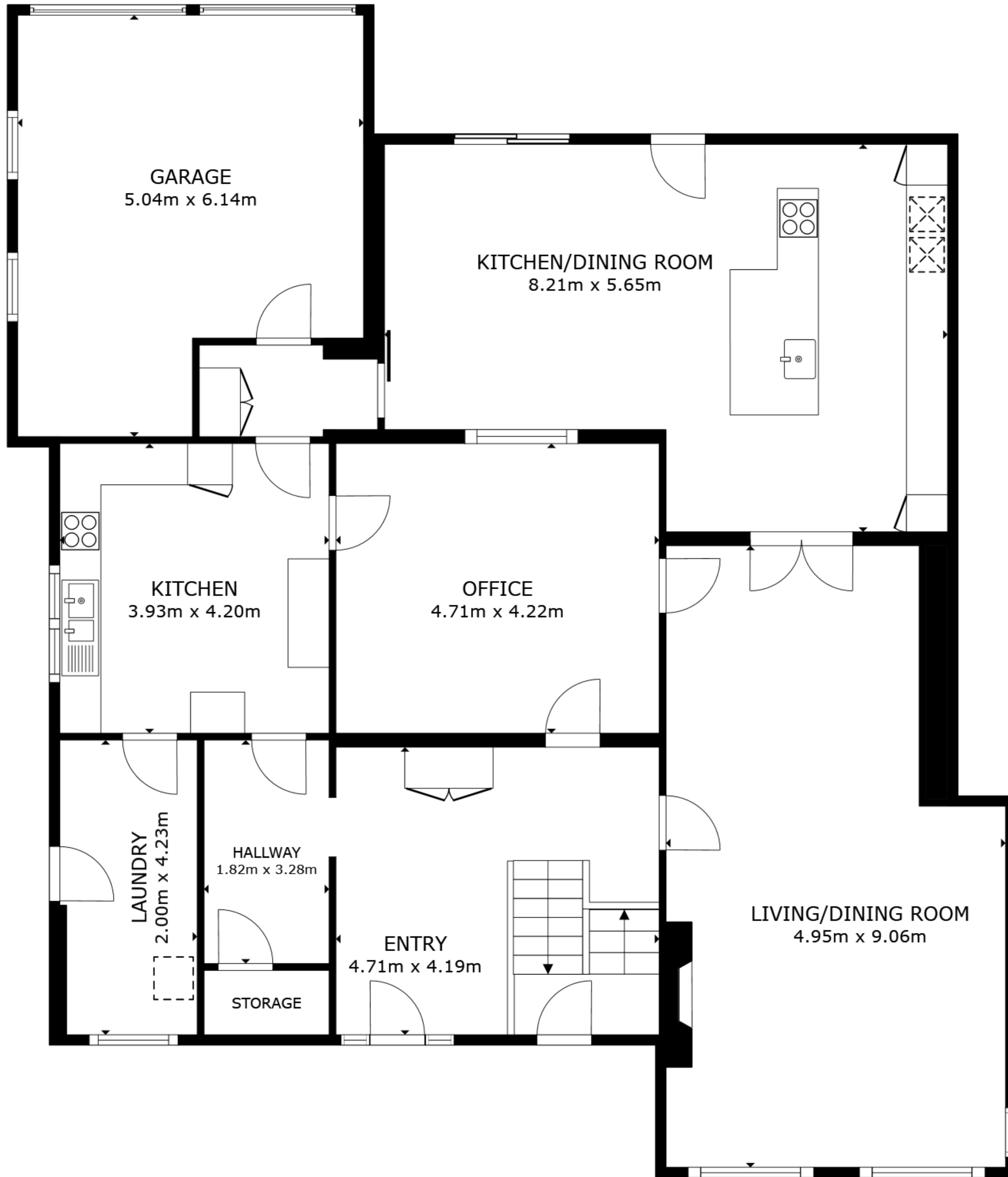
FLOOR 1
