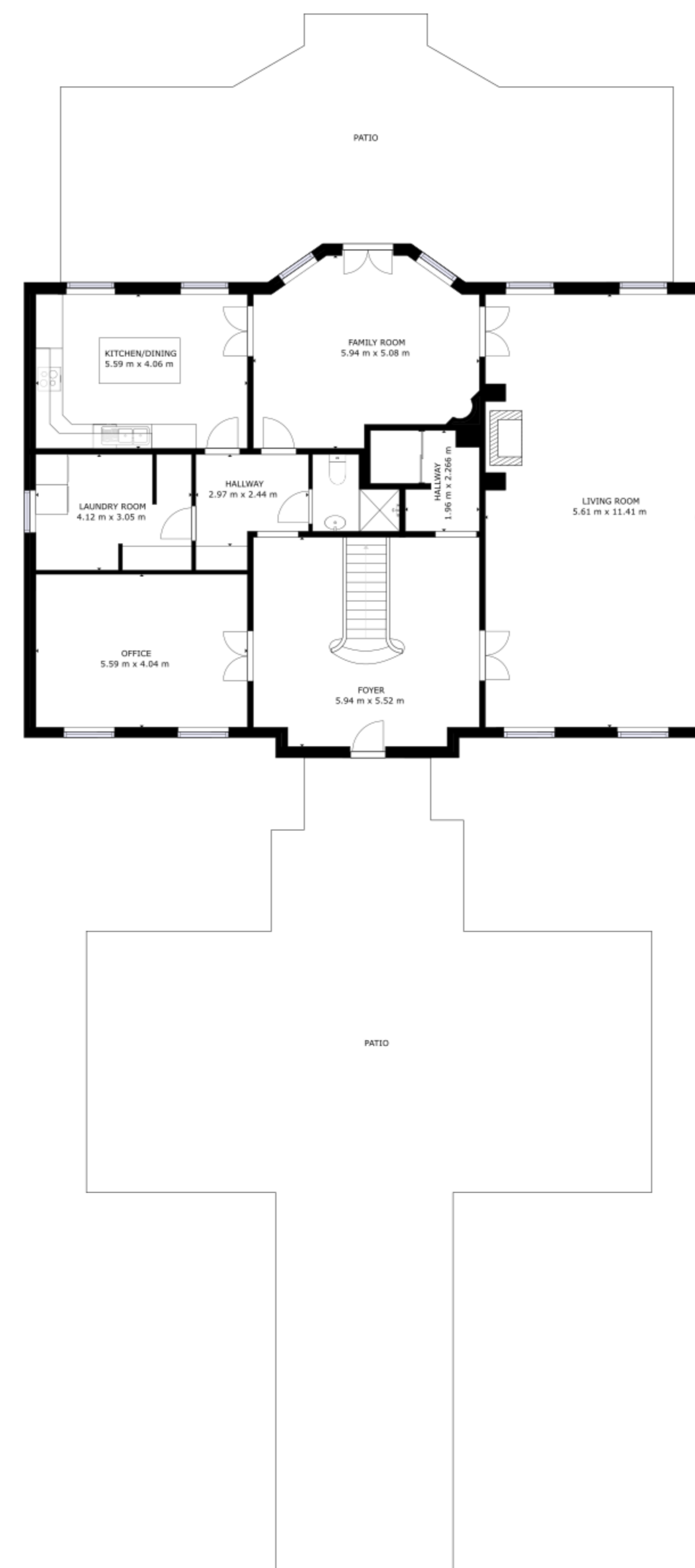
FLOOR 1
