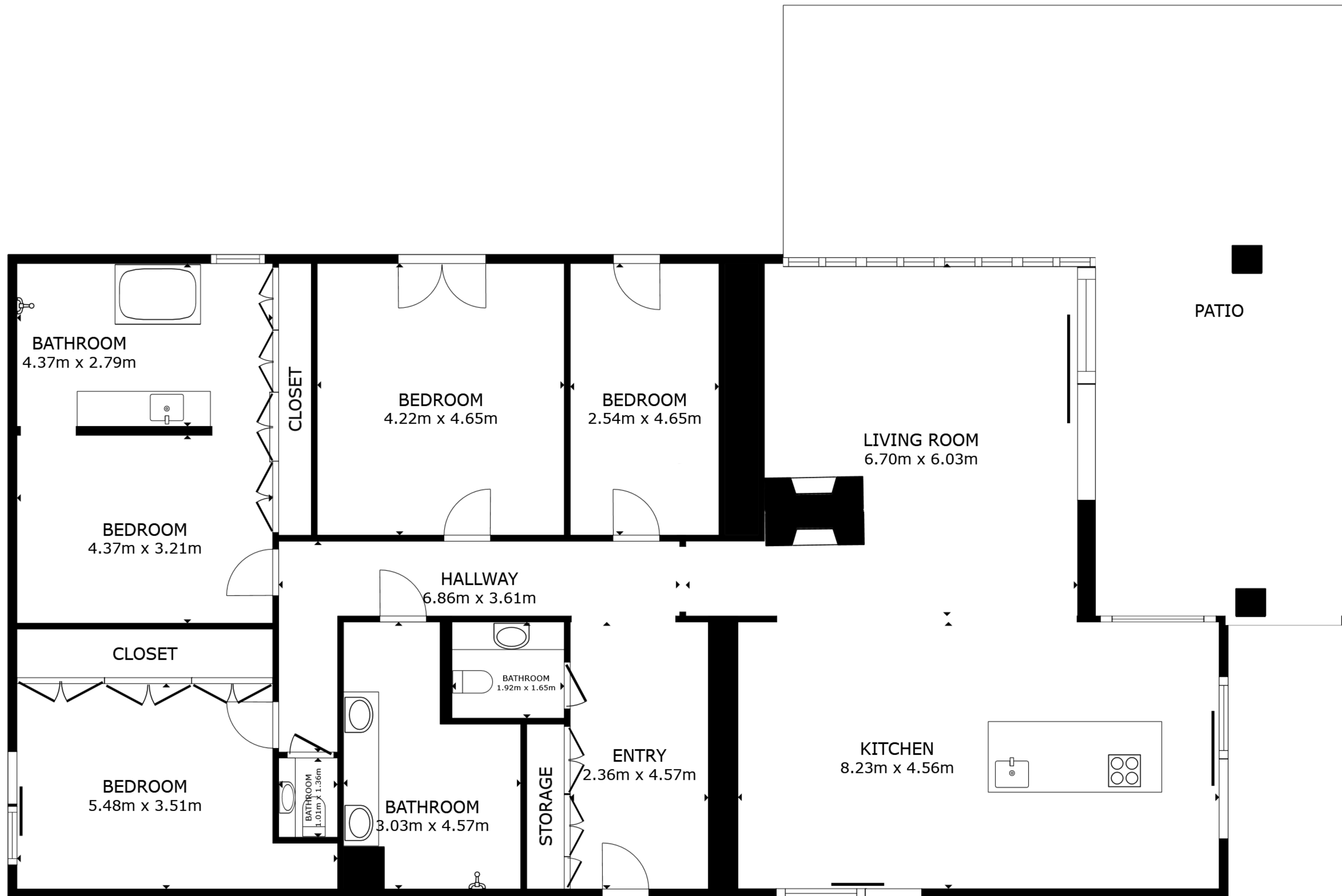
FLOOR PLAN
