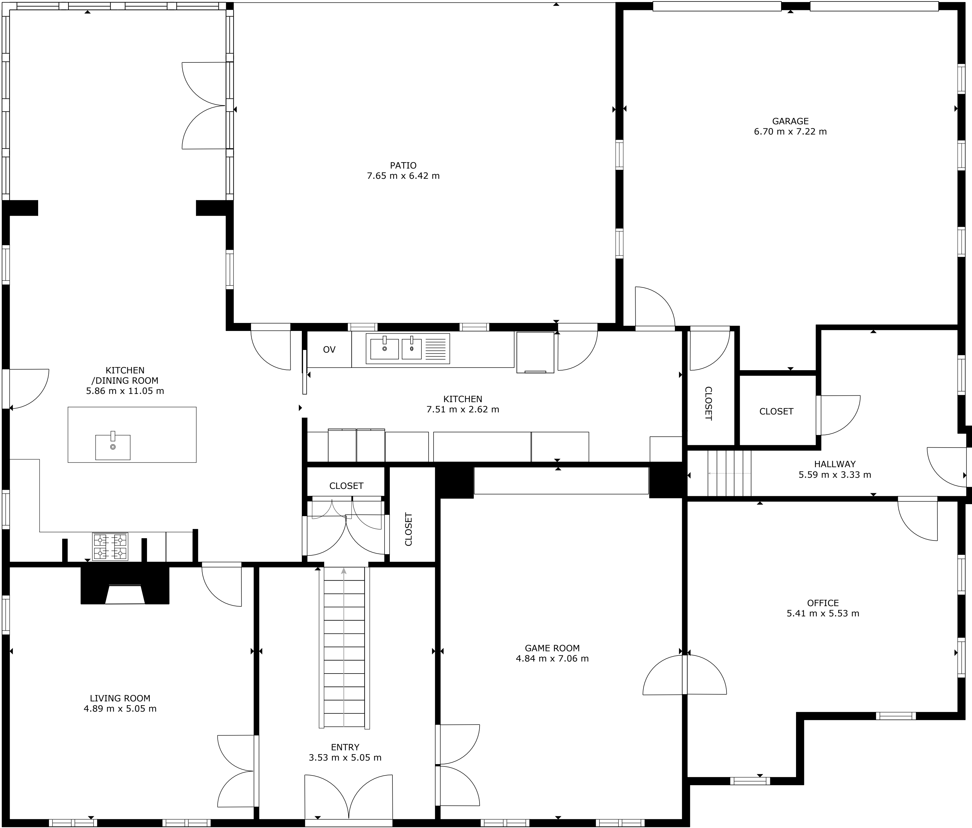
FLOOR 1
