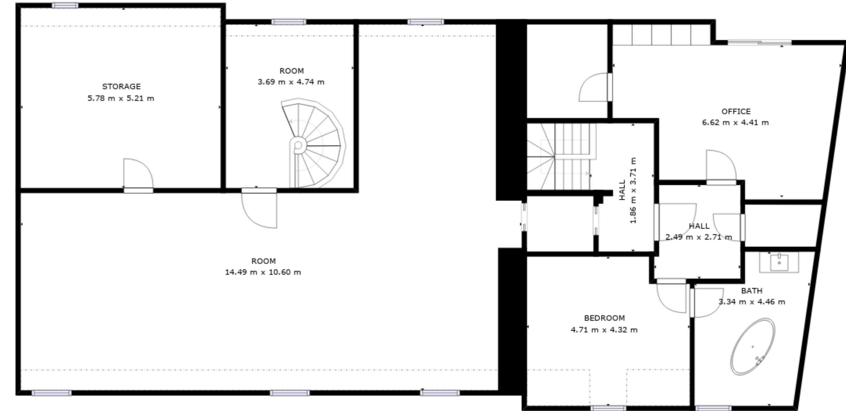
FLOOR 3
