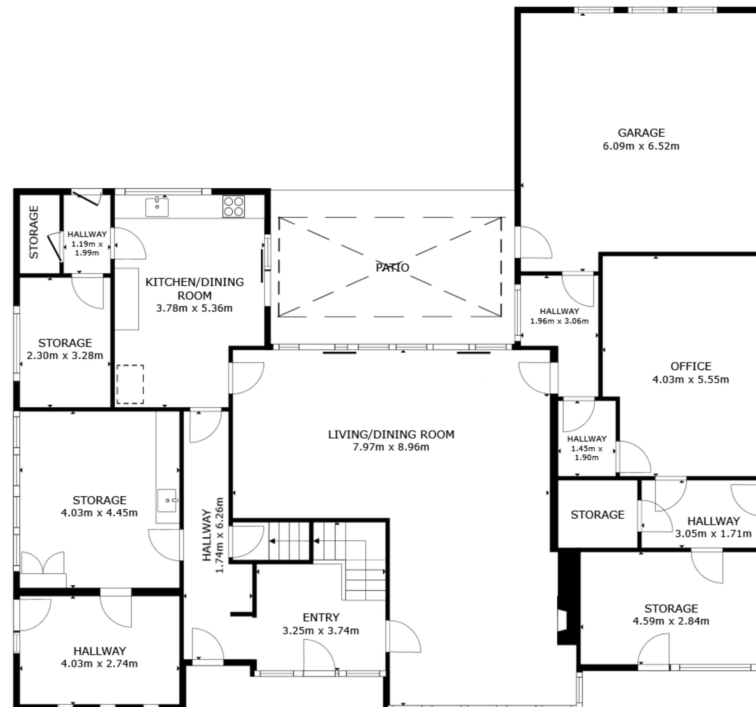
FLOOR 2
