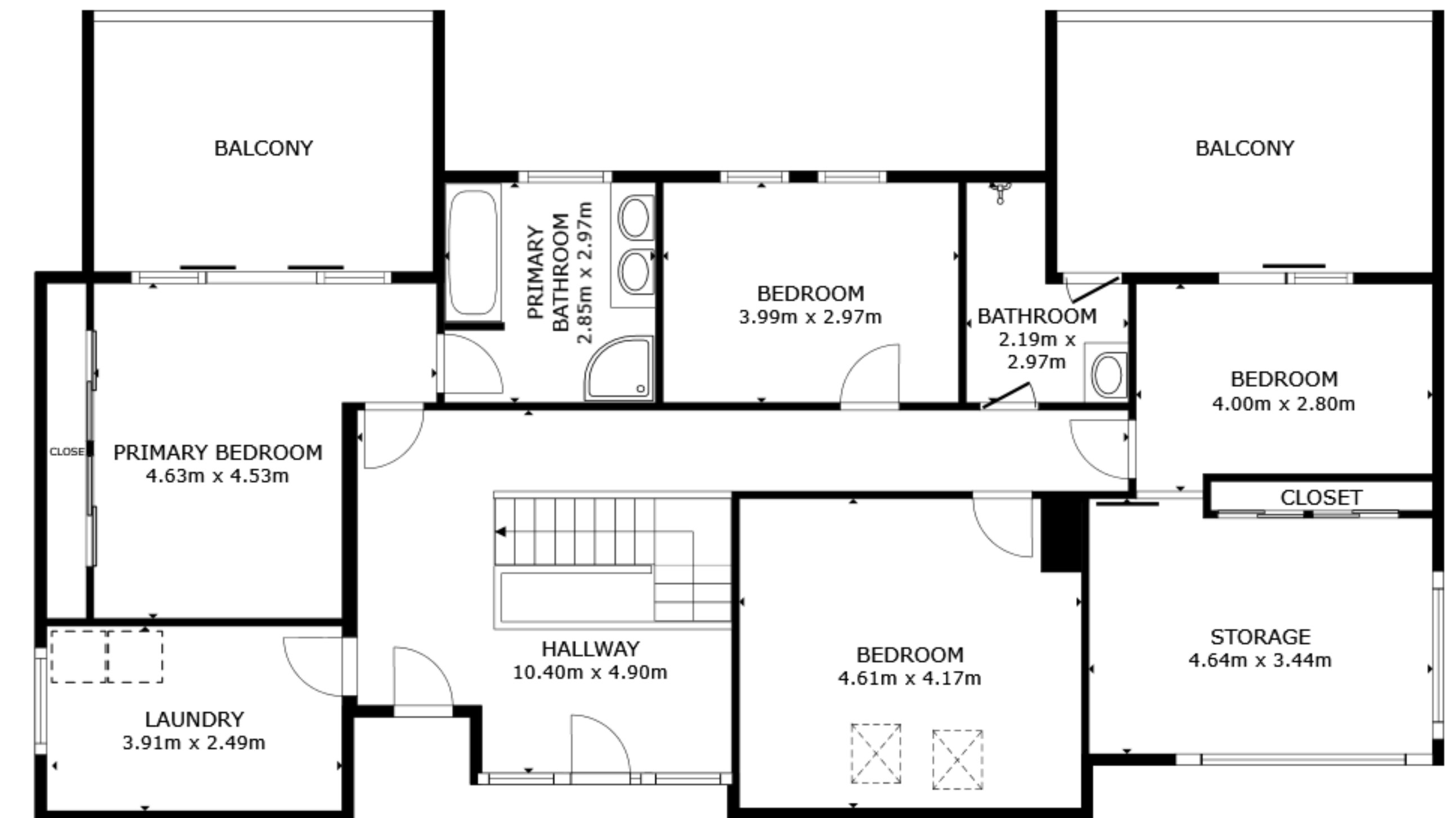
FLOOR 3
