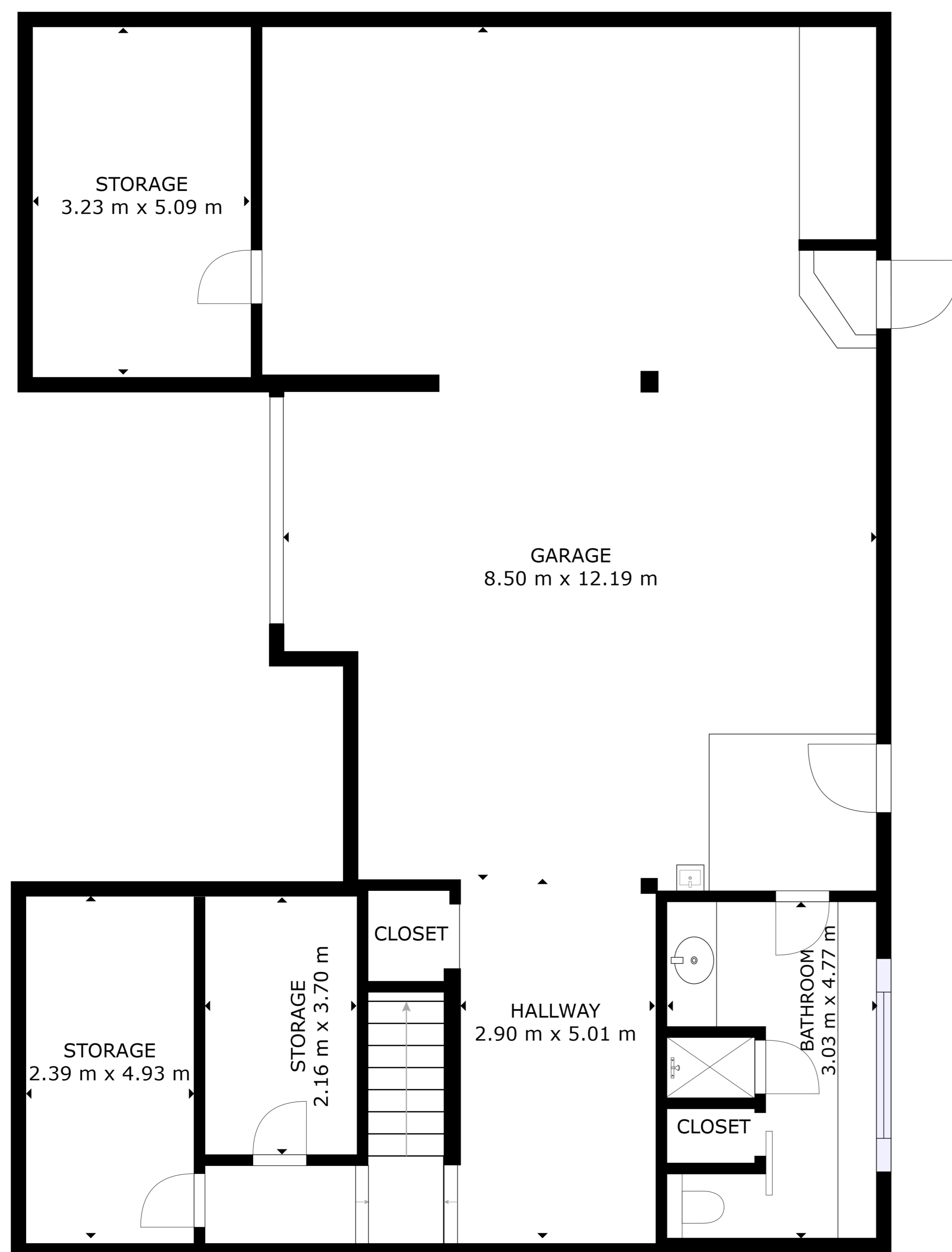
FLOOR 1
