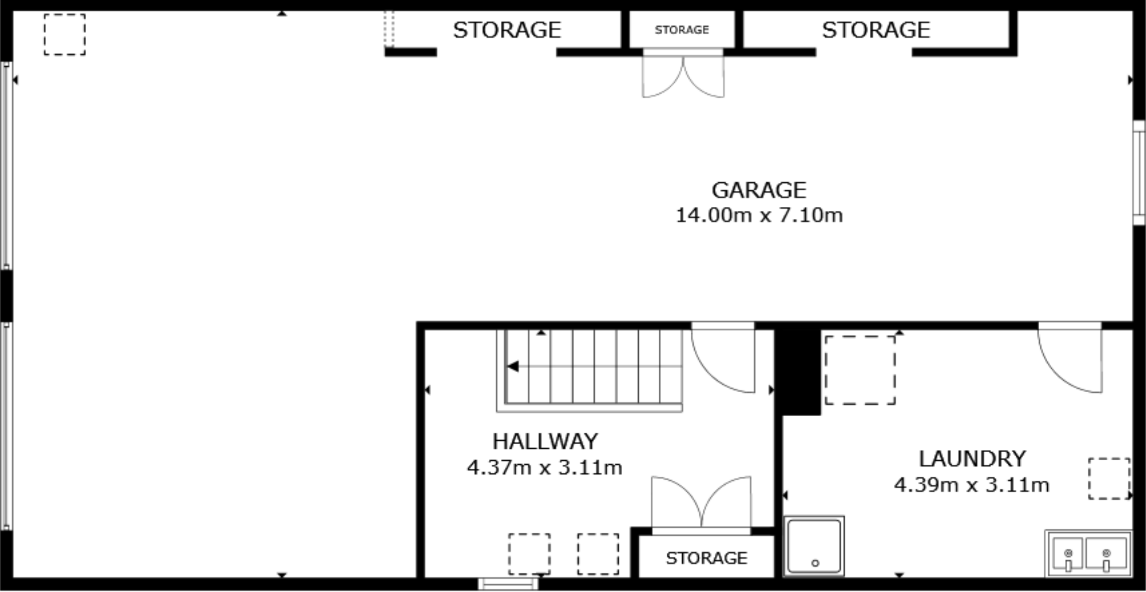
FLOOR 1
