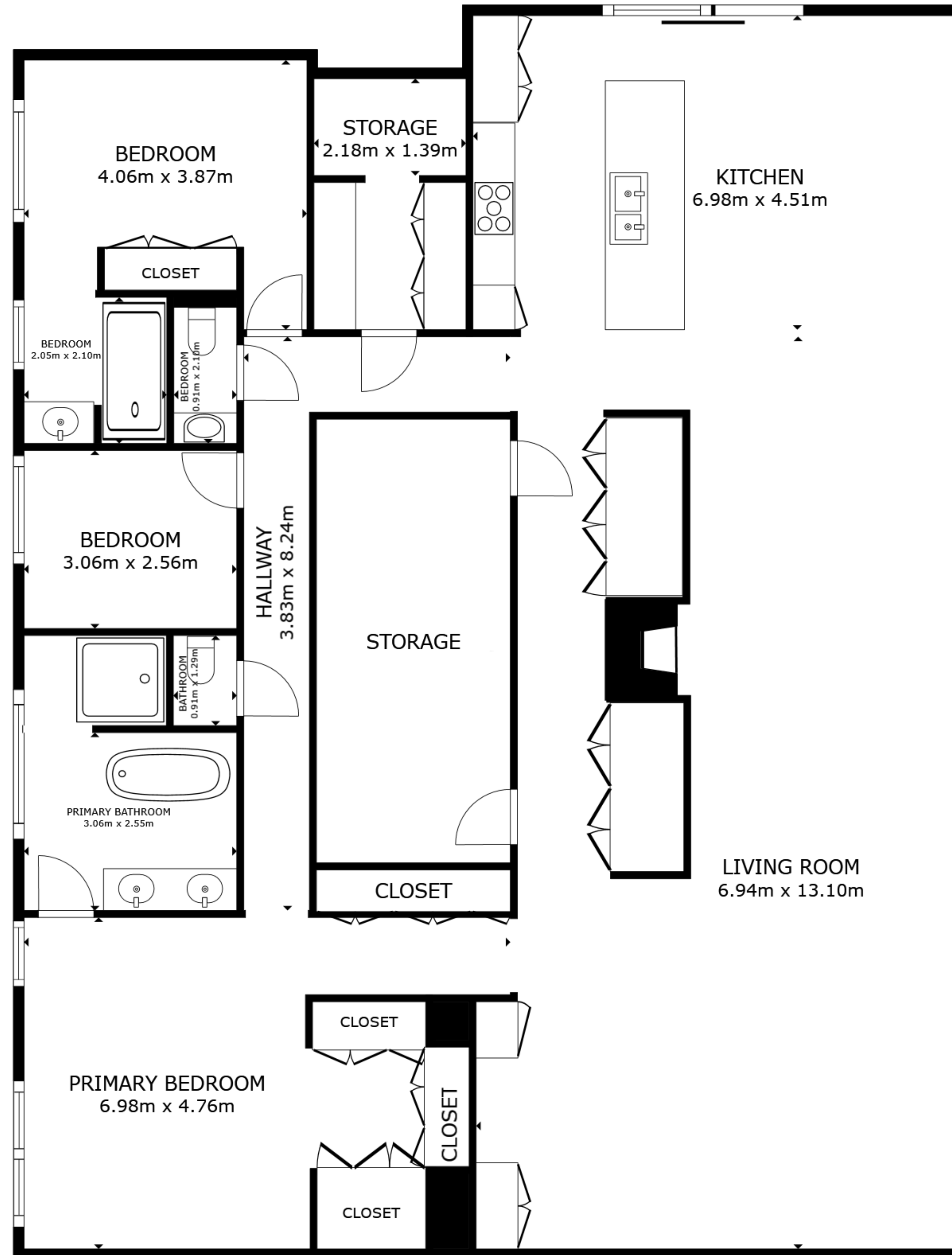
FLOOR PLAN
