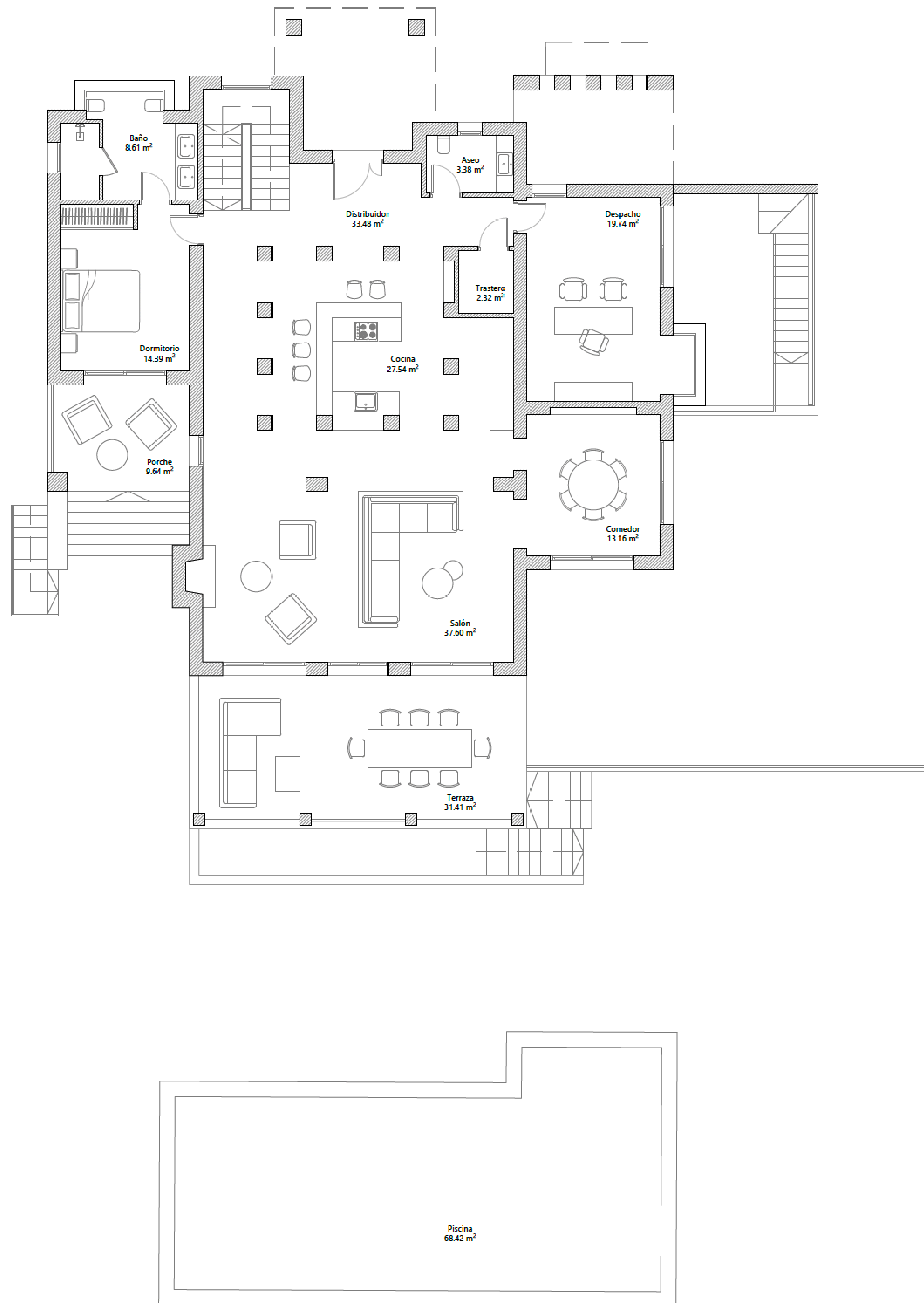
PLANTA BAJA / GROUND FLOOR
