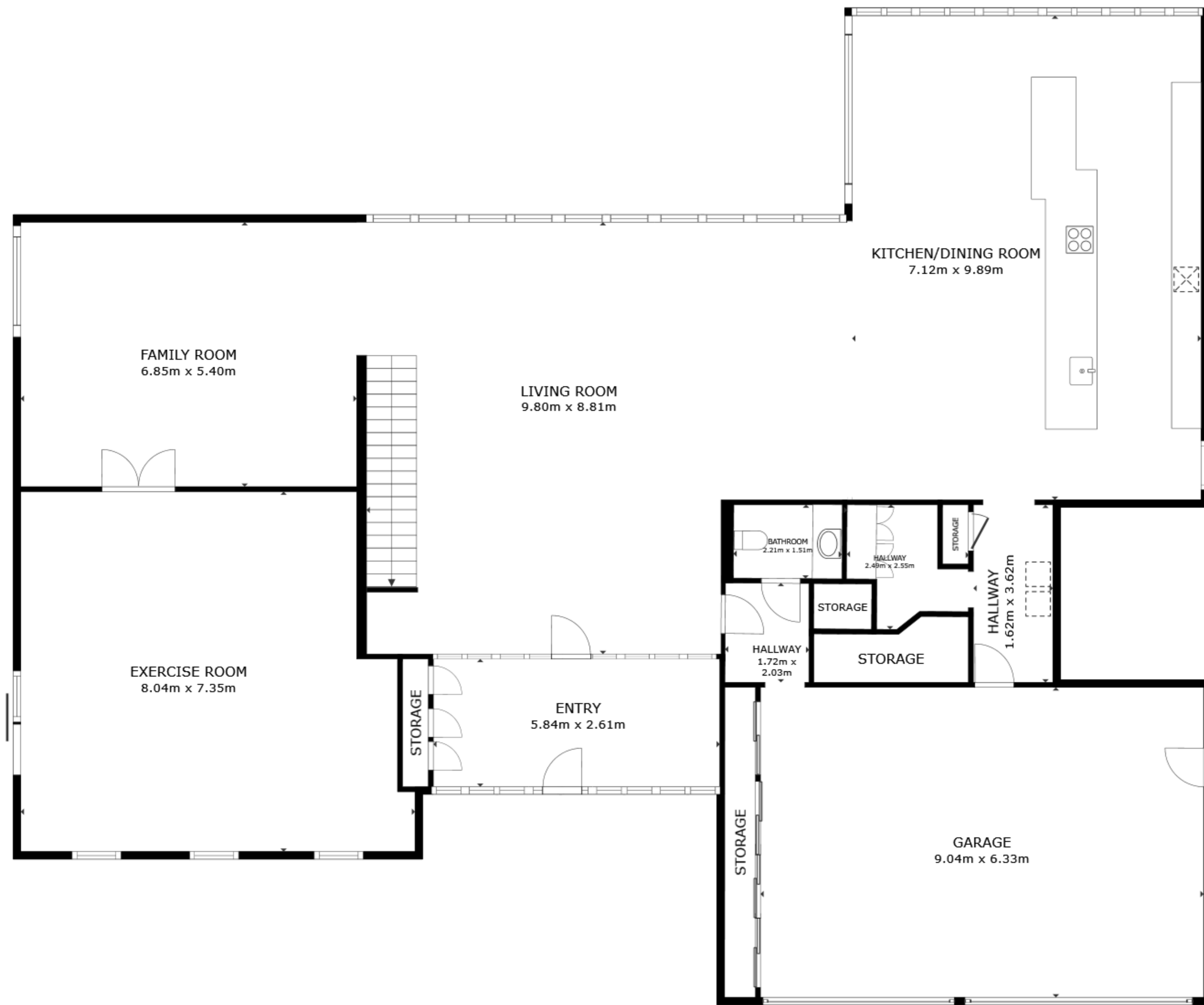
FLOOR 1
