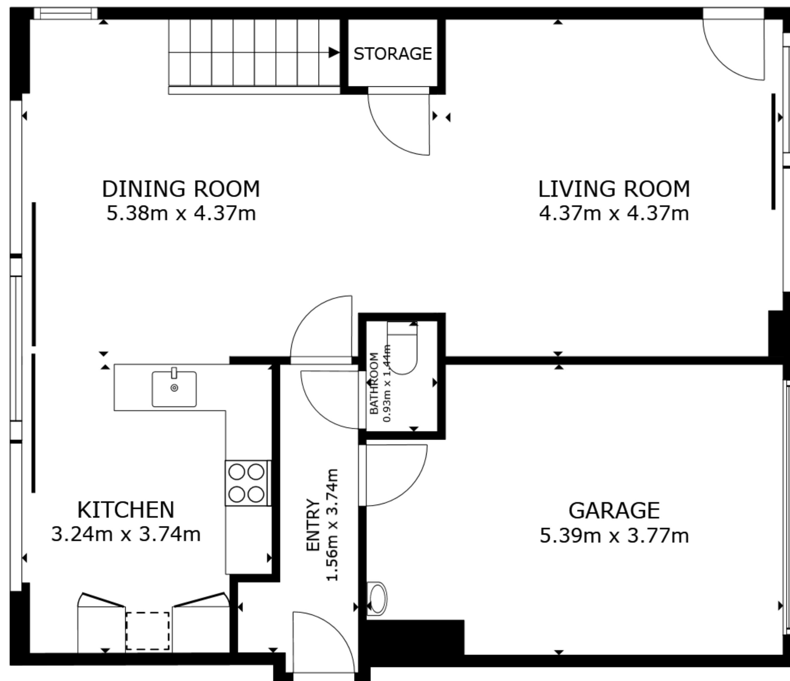
FLOOR 1
